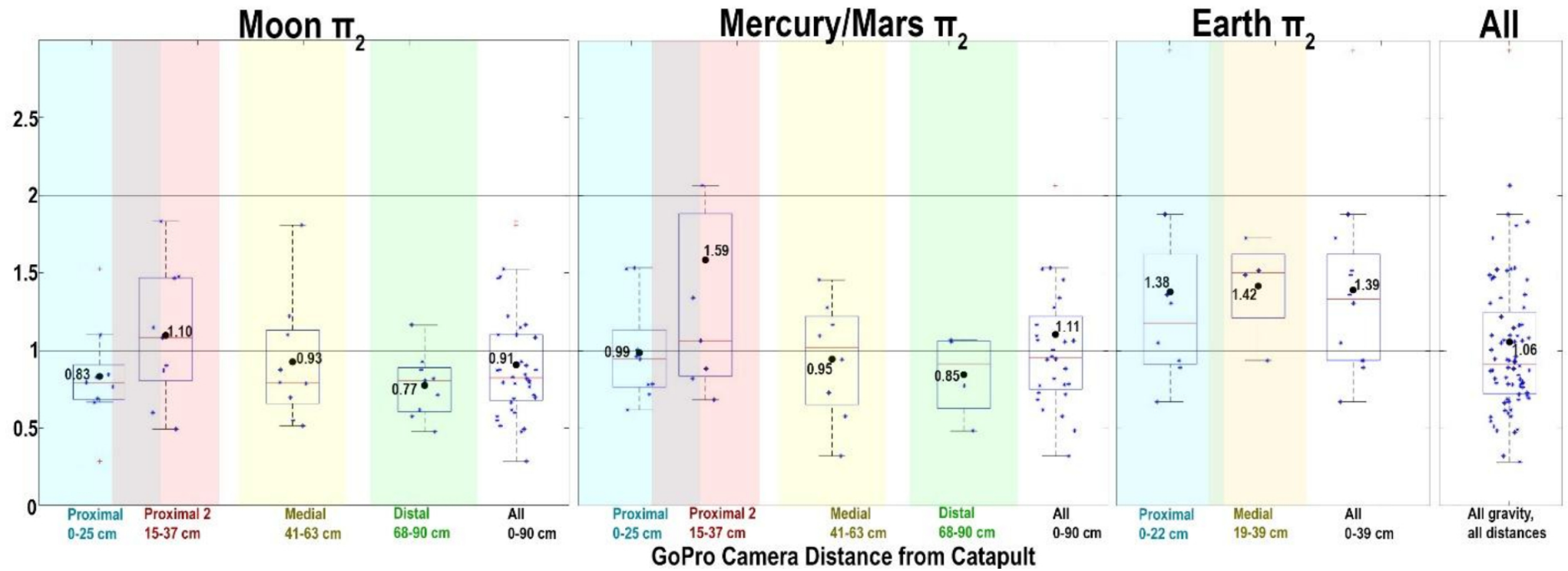
Figure 8. from Kirby D. Runyon et al 2026 Planet. Sci. J. 7 doi:10.3847/PSJ/ae9875 https://dx.doi.org/10.3847/PSJ/ae9875 © 2026. The Author(s). Published by the American Astronomical Society.
