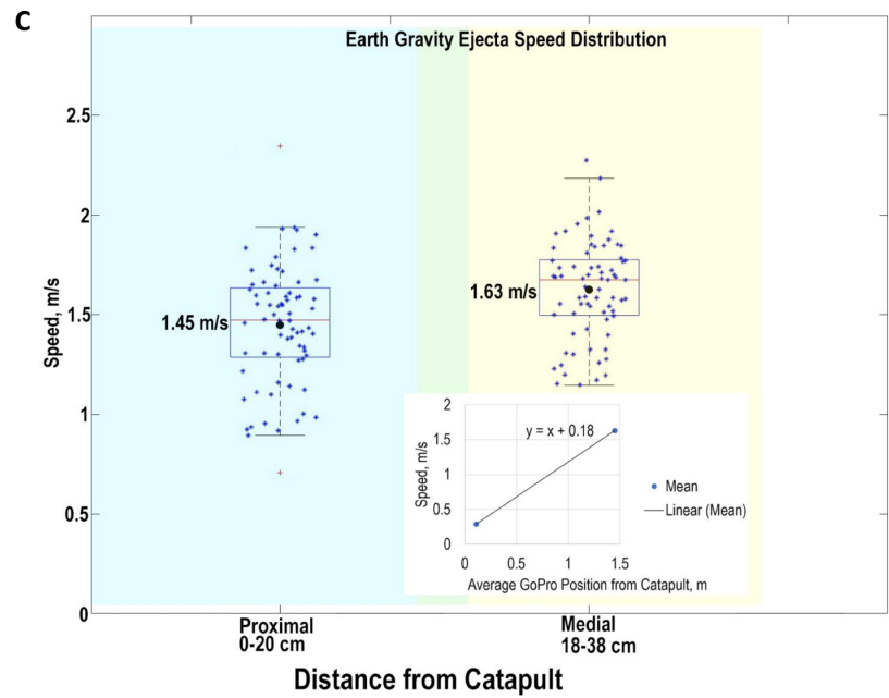
Figure 4. from Kirby D. Runyon et al 2026 Planet. Sci. J. 7 doi:10.3847/PSJ/ae9875 https://dx.doi.org/10.3847/PSJ/ae9875 © 2026. The Author(s). Published by the American Astronomical Society.
