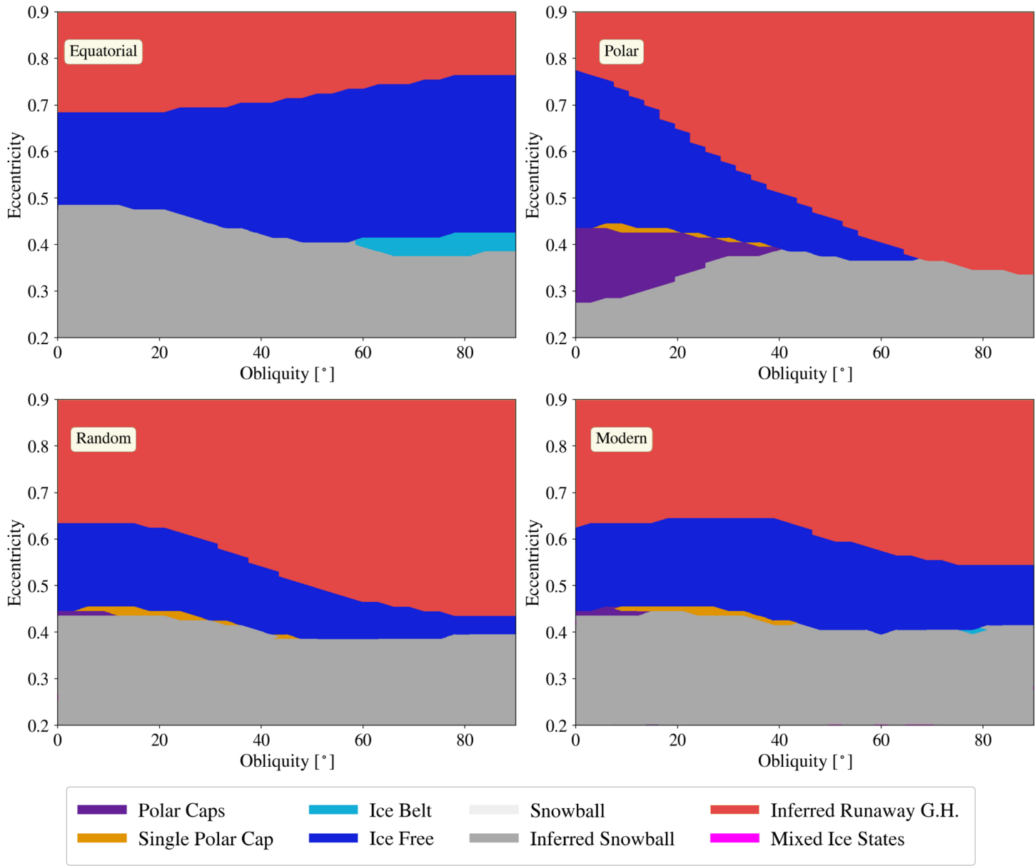
Figure 9. from Héctor E. Delgado Díaz et al 2026 Planet. Sci. J. 7 doi:10.3847/PSJ/ae9861 https://dx.doi.org/10.3847/PSJ/ae9861 © 2026. The Author(s). Published by the American Astronomical Society.
