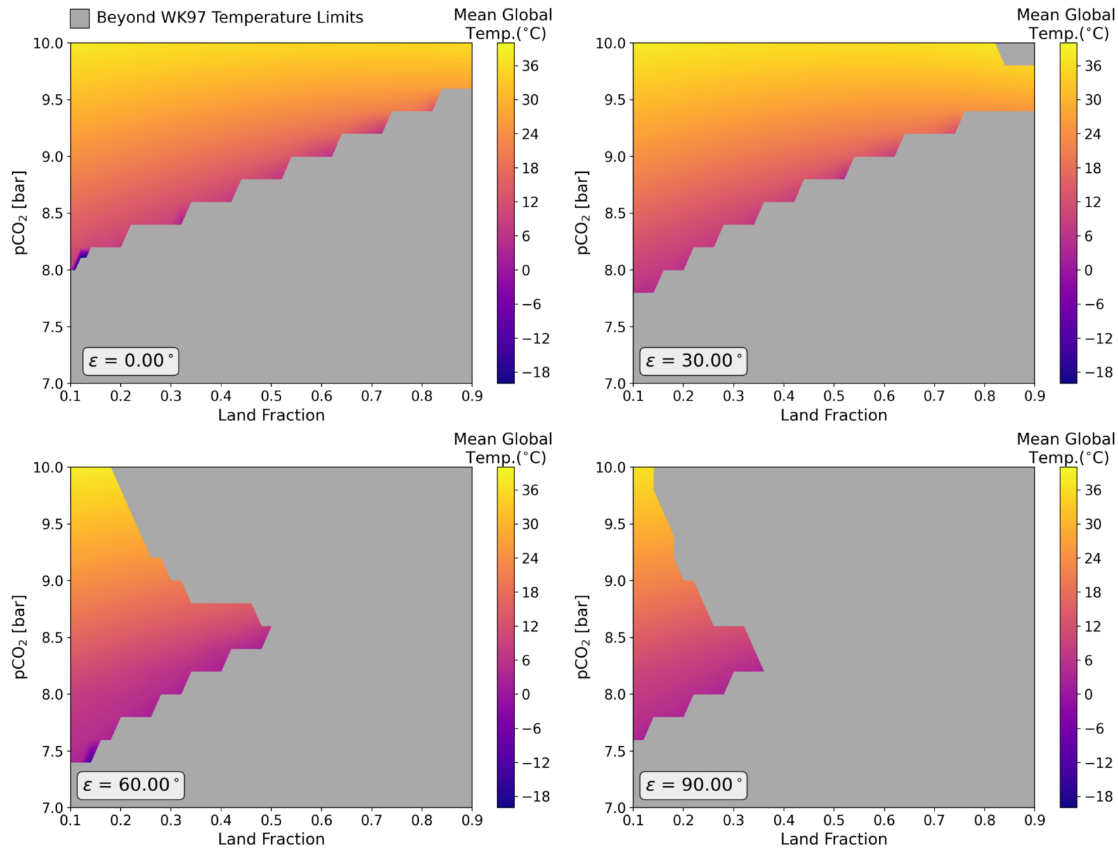
Figure 7. from Héctor E. Delgado Díaz et al 2026 Planet. Sci. J. 7 doi:10.3847/PSJ/ae9861 https://dx.doi.org/10.3847/PSJ/ae9861 © 2026. The Author(s). Published by the American Astronomical Society.
