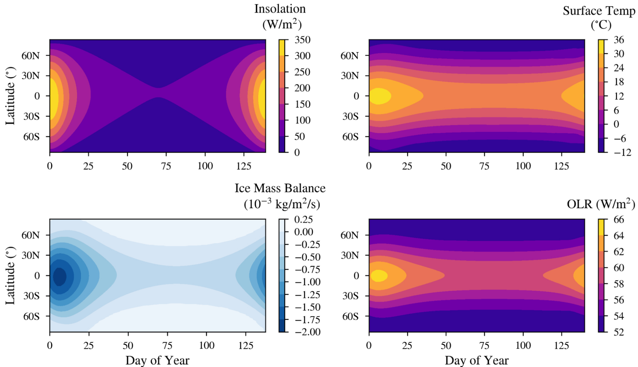
Figure 3. from Héctor E. Delgado Díaz et al 2026 Planet. Sci. J. 7 doi:10.3847/PSJ/ae9861 https://dx.doi.org/10.3847/PSJ/ae9861 © 2026. The Author(s). Published by the American Astronomical Society.
