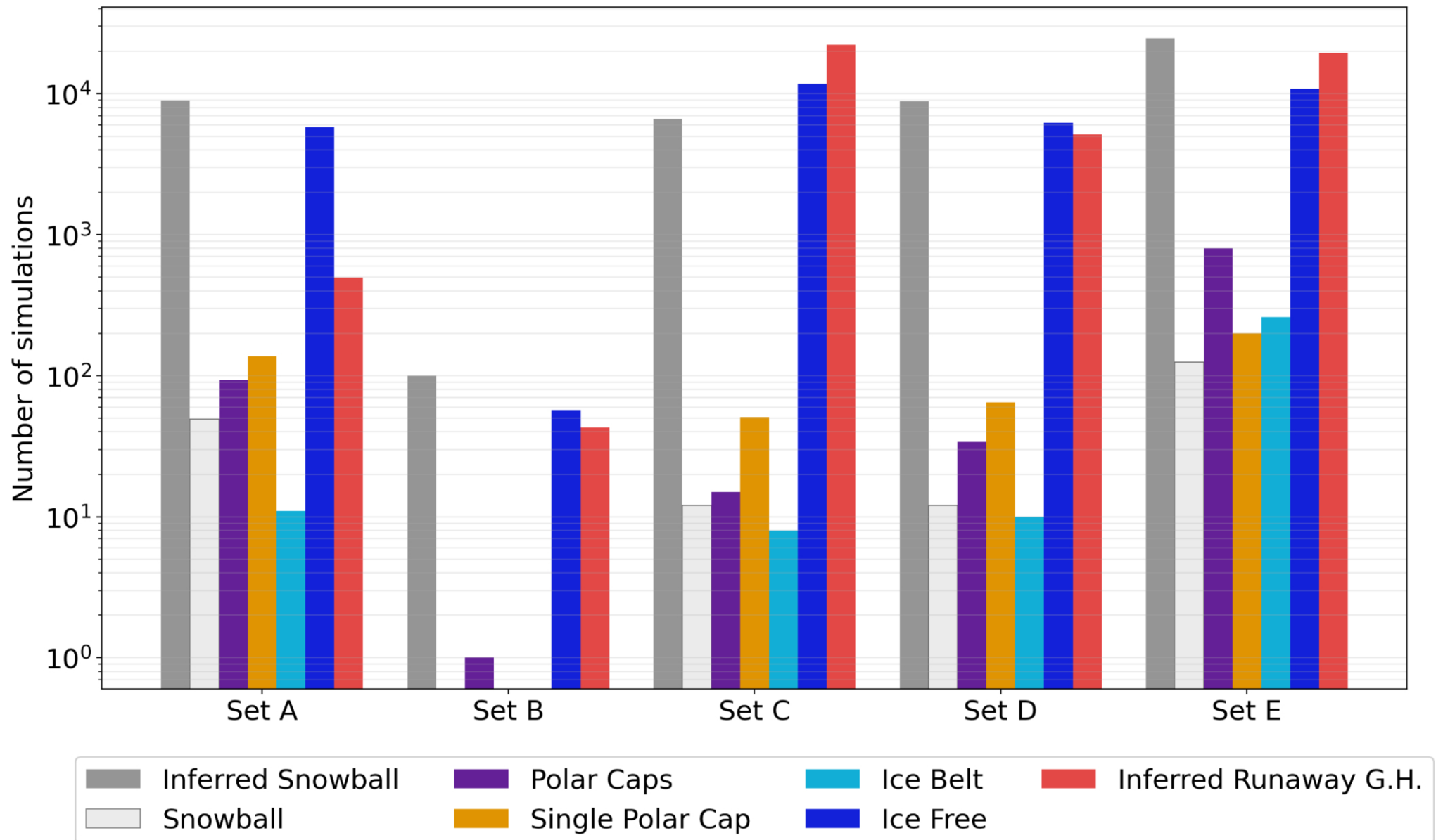
Figure 10. from Héctor E. Delgado Díaz et al 2026 Planet. Sci. J. 7 doi:10.3847/PSJ/ae9861 https://dx.doi.org/10.3847/PSJ/ae9861 © 2026. The Author(s). Published by the American Astronomical Society.
