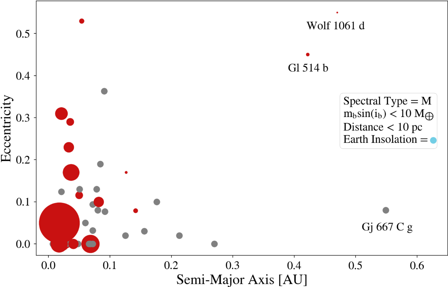
Figure 1. from Héctor E. Delgado Díaz et al 2026 Planet. Sci. J. 7 doi:10.3847/PSJ/ae9861 https://dx.doi.org/10.3847/PSJ/ae9861 © 2026. The Author(s). Published by the American Astronomical Society.
