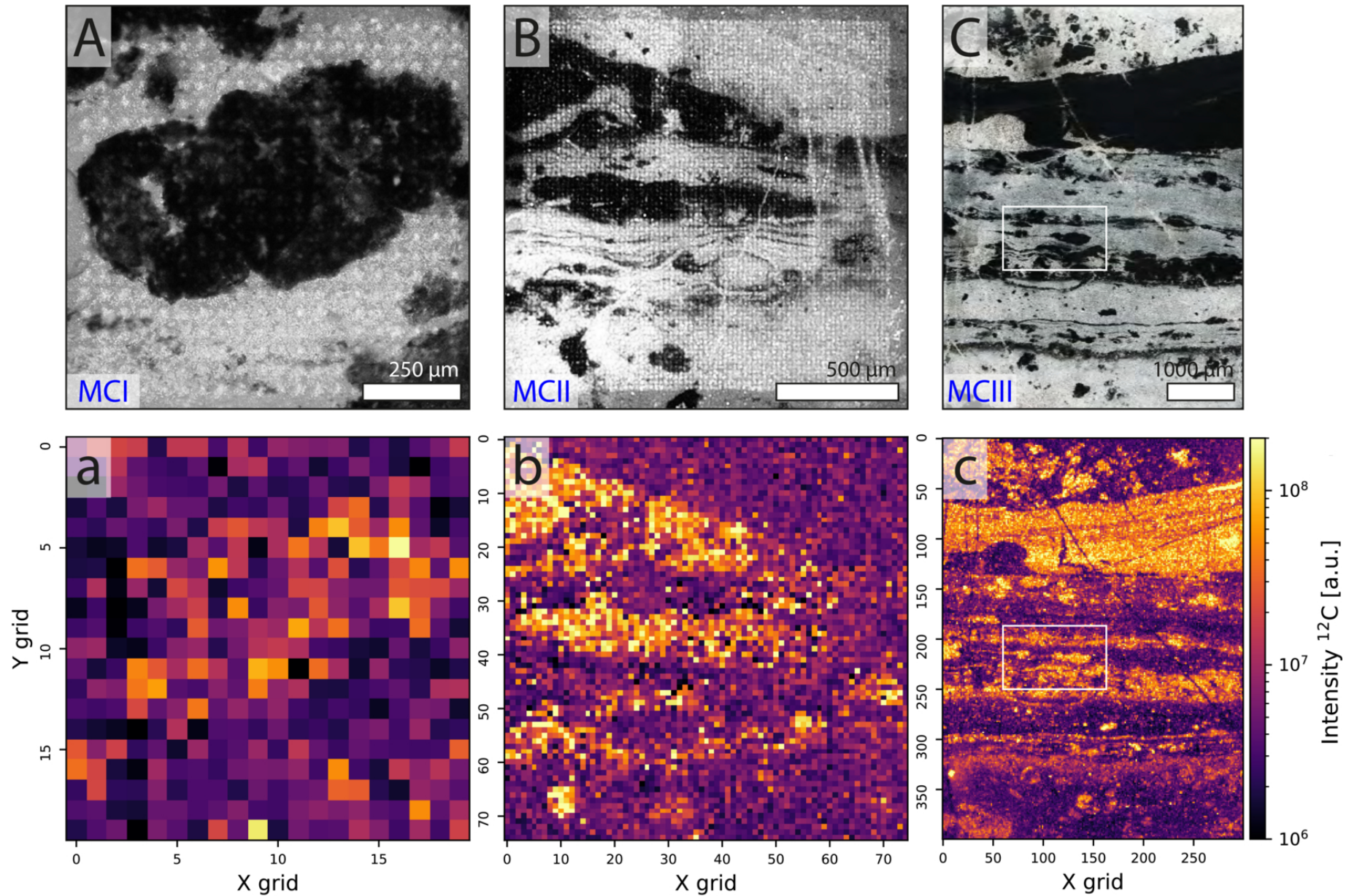
Figure 9. from Salome Gruchola et al 2026 Planet. Sci. J. 7 doi:10.3847/PSJ/ae9839 https://dx.doi.org/10.3847/PSJ/ae9839 © 2026. The Author(s). Published by the American Astronomical Society.
