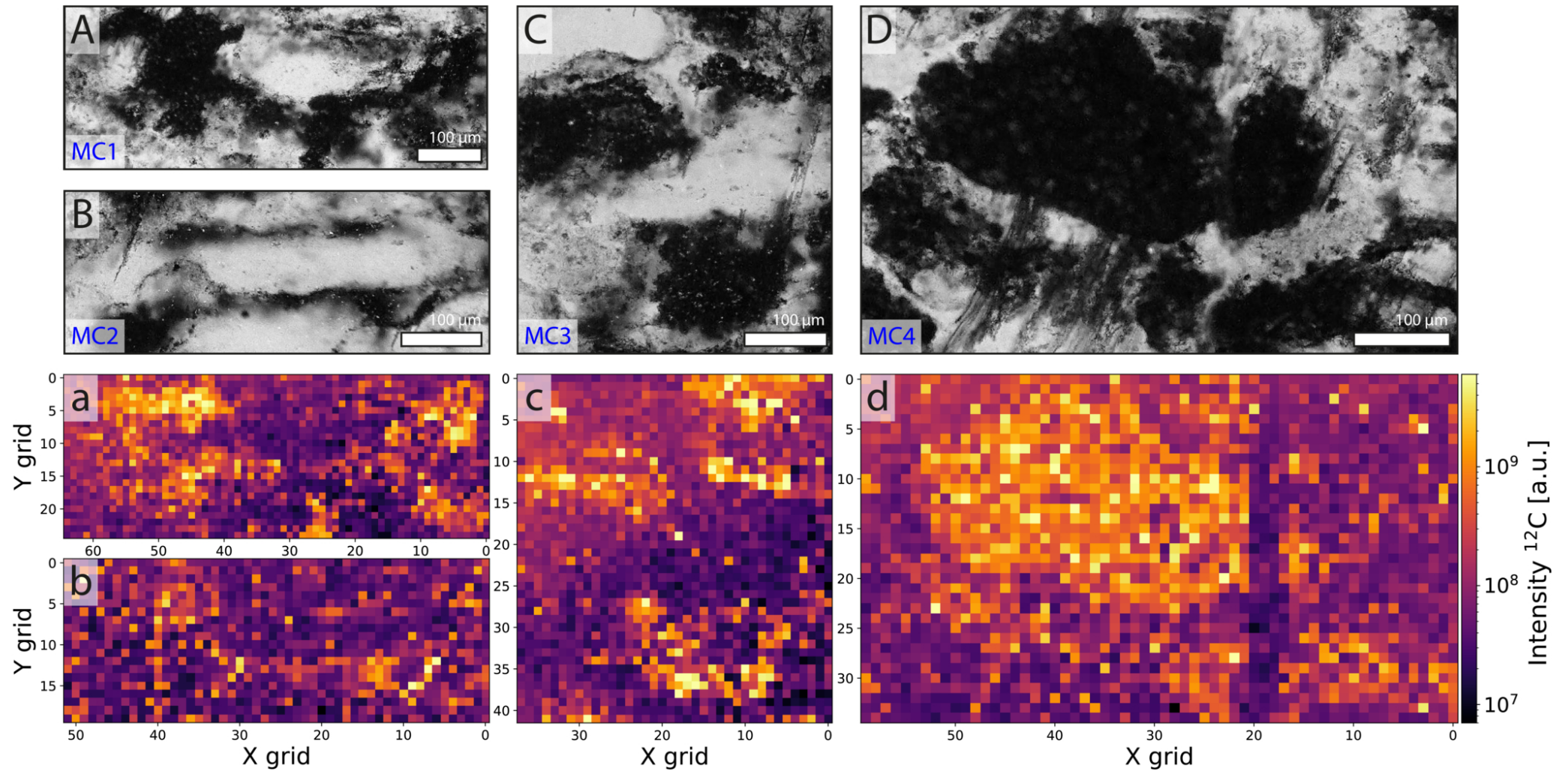
Figure 5. from Salome Gruchola et al 2026 Planet. Sci. J. 7 doi:10.3847/PSJ/ae9839 https://dx.doi.org/10.3847/PSJ/ae9839 © 2026. The Author(s). Published by the American Astronomical Society.
