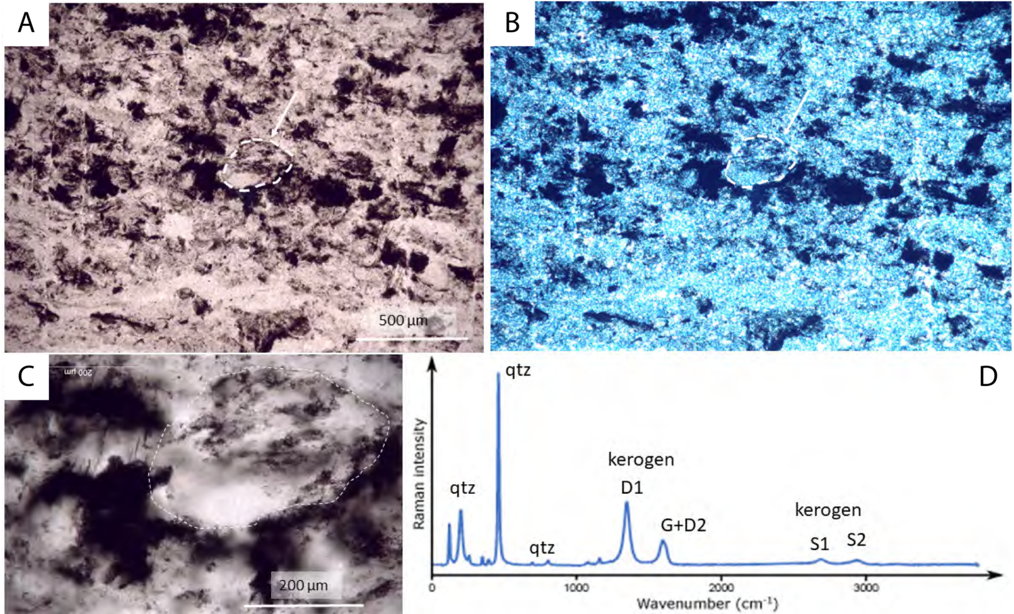
Figure C2. from Salome Gruchola et al 2026 Planet. Sci. J. 7 doi:10.3847/PSJ/ae9839 https://dx.doi.org/10.3847/PSJ/ae9839 © 2026. The Author(s). Published by the American Astronomical Society.
