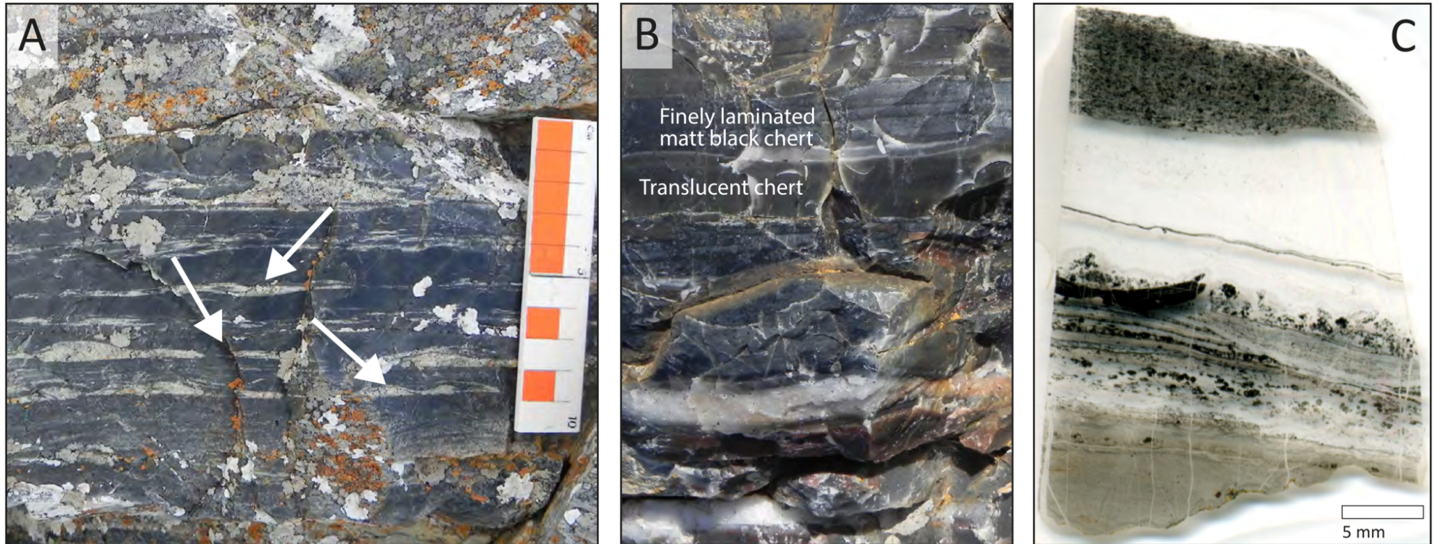
Figure 1. from Salome Gruchola et al 2026 Planet. Sci. J. 7 doi:10.3847/PSJ/ae9839 https://dx.doi.org/10.3847/PSJ/ae9839 © 2026. The Author(s). Published by the American Astronomical Society.
