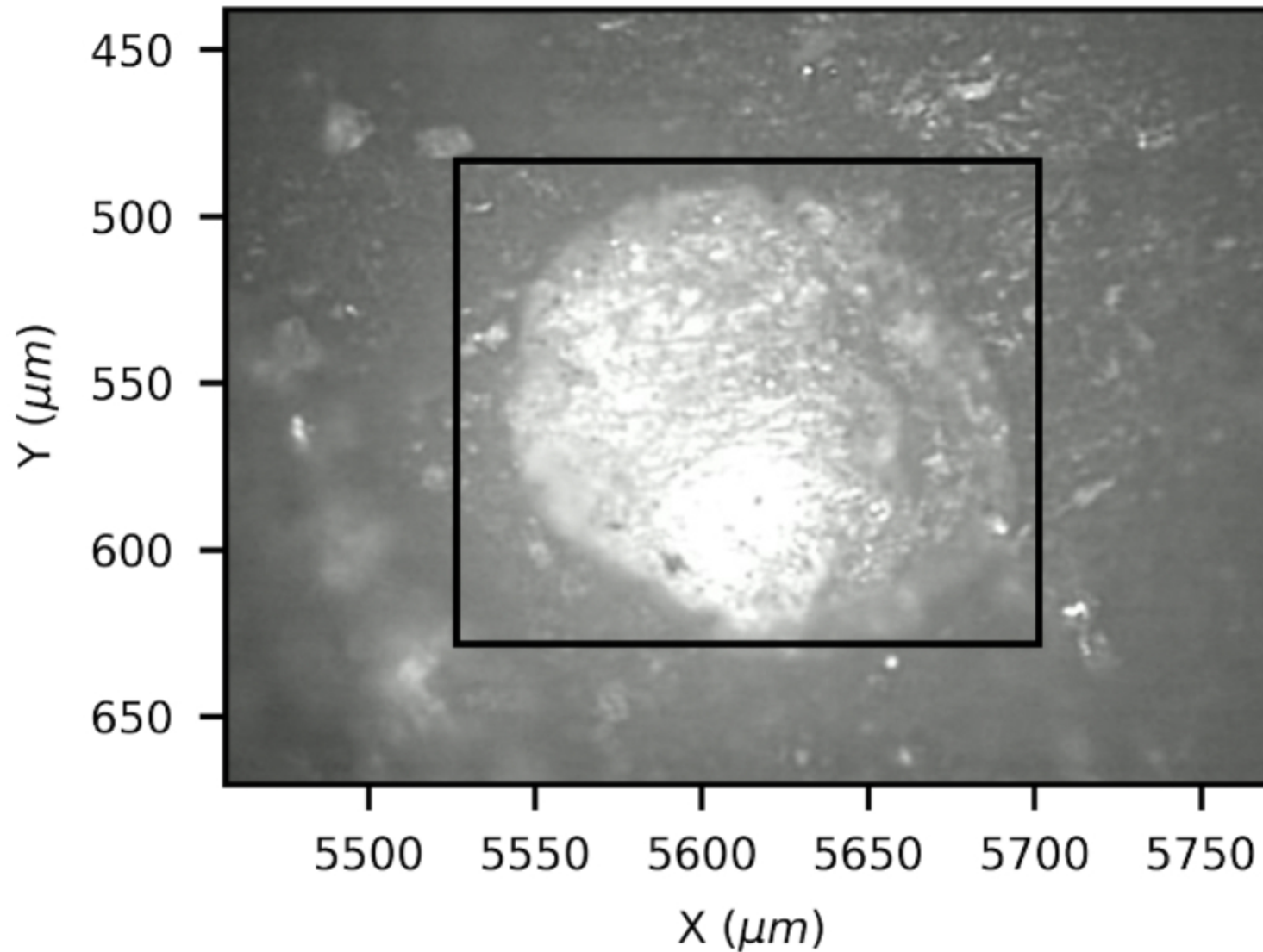
Figure 8. from Lorraine Roselló Del Valle et al 2026 Planet. Sci. J. 7 doi:10.3847/PSJ/ae96b5 https://dx.doi.org/10.3847/PSJ/ae96b5 © 2026. The Author(s). Published by the American Astronomical Society.
