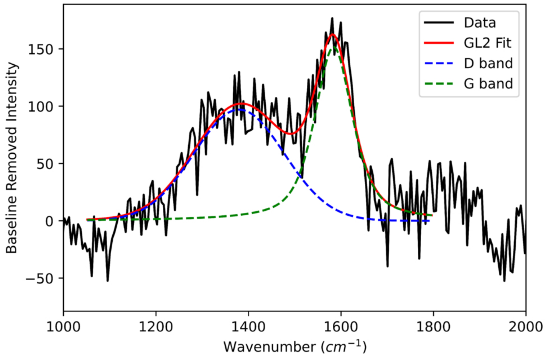
Figure 4. from Lorraine Roselló Del Valle et al 2026 Planet. Sci. J. 7 doi:10.3847/PSJ/ae96b5 https://dx.doi.org/10.3847/PSJ/ae96b5 © 2026. The Author(s). Published by the American Astronomical Society.
