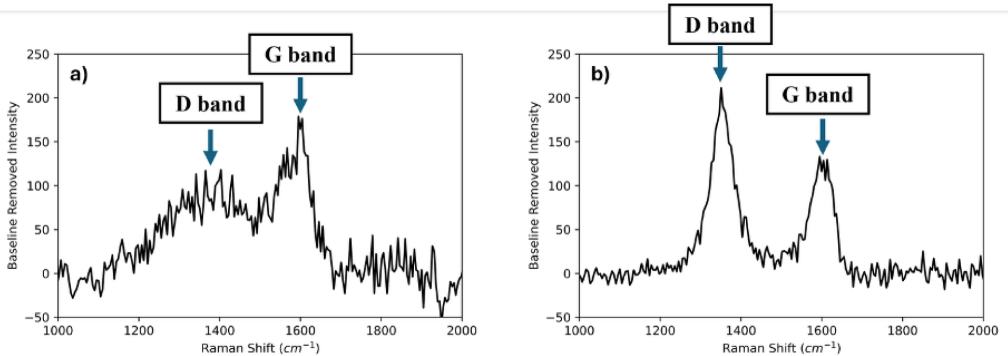
Figure 3. from Lorraine Roselló Del Valle et al 2026 Planet. Sci. J. 7 doi:10.3847/PSJ/ae96b5 https://dx.doi.org/10.3847/PSJ/ae96b5 © 2026. The Author(s). Published by the American Astronomical Society.
