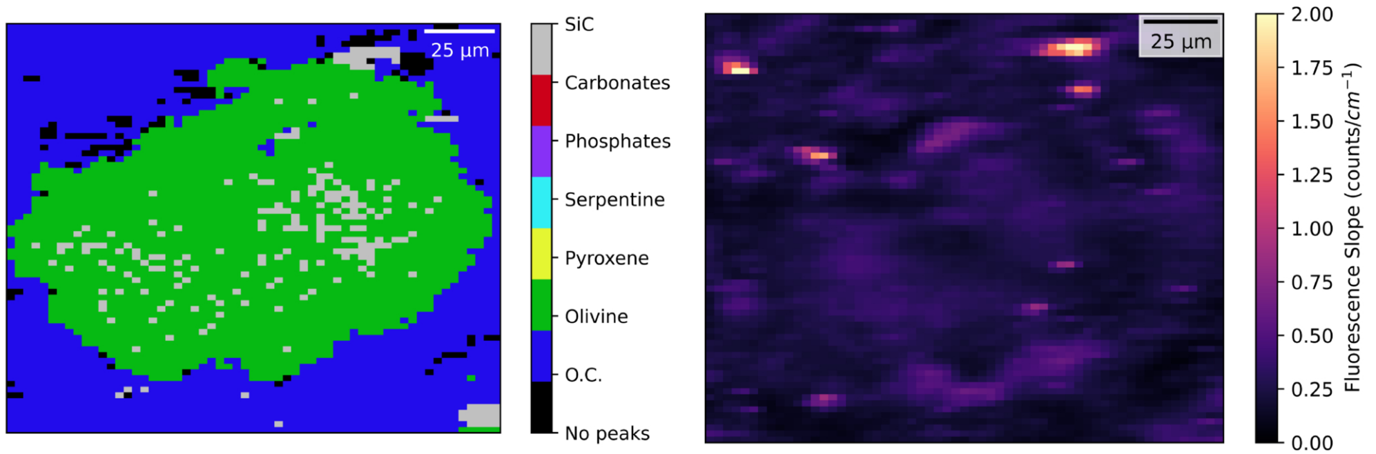
Figure 18. from Lorraine Roselló Del Valle et al 2026 Planet. Sci. J. 7 doi:10.3847/PSJ/ae96b5 https://dx.doi.org/10.3847/PSJ/ae96b5 © 2026. The Author(s). Published by the American Astronomical Society.
