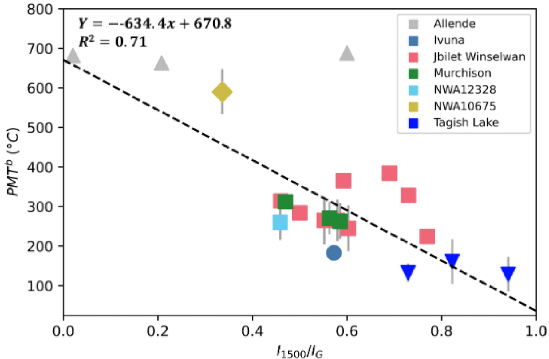
Figure 16. from Lorraine Roselló Del Valle et al 2026 Planet. Sci. J. 7 doi:10.3847/PSJ/ae96b5 https://dx.doi.org/10.3847/PSJ/ae96b5 © 2026. The Author(s). Published by the American Astronomical Society.
