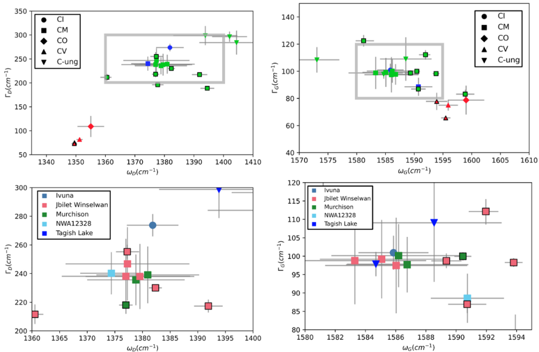
Figure 14. from Lorraine Roselló Del Valle et al 2026 Planet. Sci. J. 7 doi:10.3847/PSJ/ae96b5 https://dx.doi.org/10.3847/PSJ/ae96b5 © 2026. The Author(s). Published by the American Astronomical Society.
