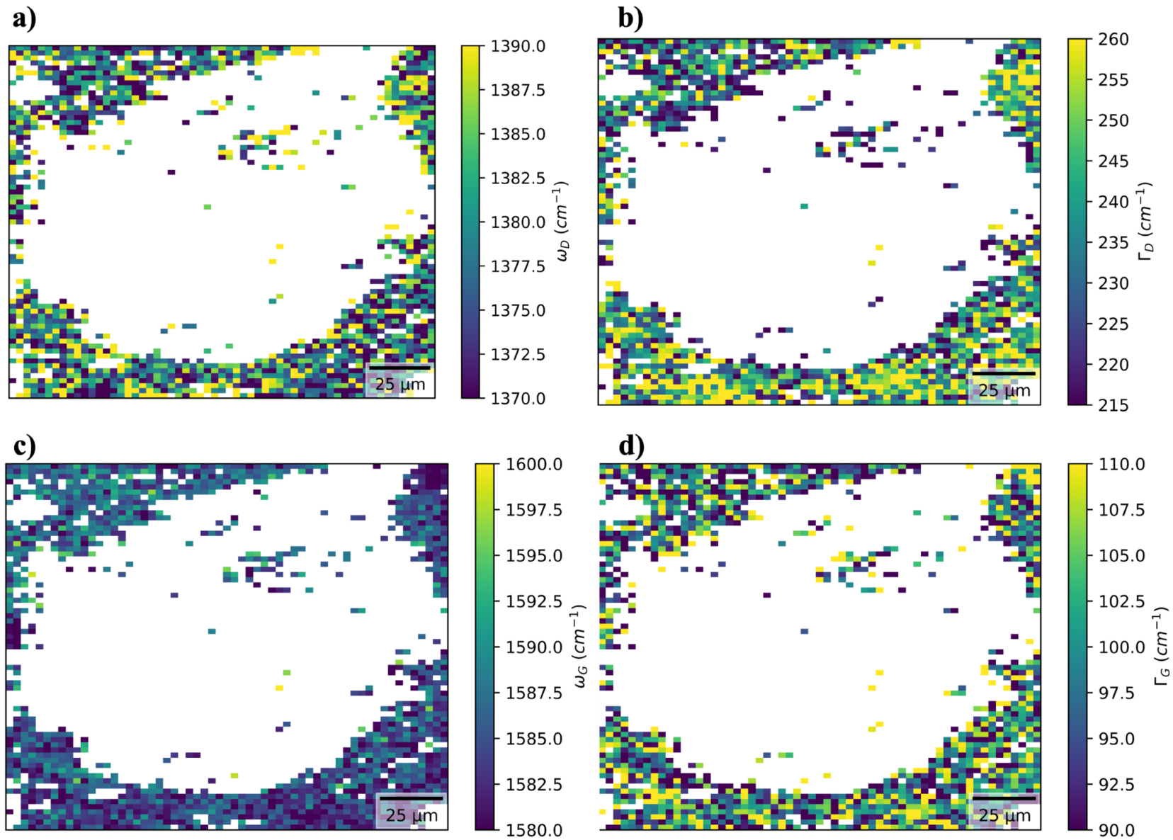
Figure 13. from Lorraine Roselló Del Valle et al 2026 Planet. Sci. J. 7 doi:10.3847/PSJ/ae96b5 https://dx.doi.org/10.3847/PSJ/ae96b5 © 2026. The Author(s). Published by the American Astronomical Society.
