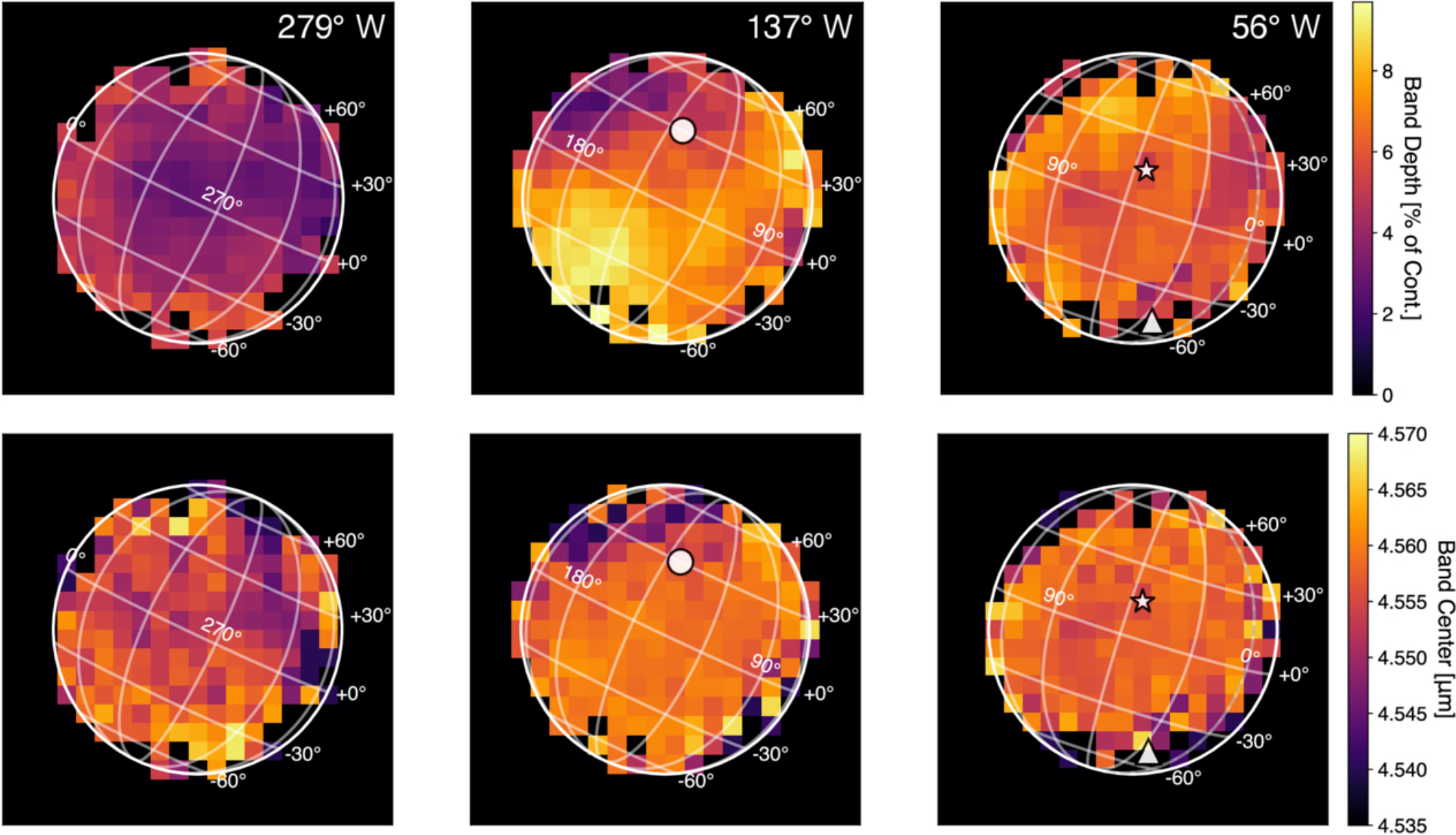
Figure 6. from Maria Camarca et al 2026 Planet. Sci. J. 7 doi:10.3847/PSJ/ae9608 https://dx.doi.org/10.3847/PSJ/ae9608 © 2026. The Author(s). Published by the American Astronomical Society.
