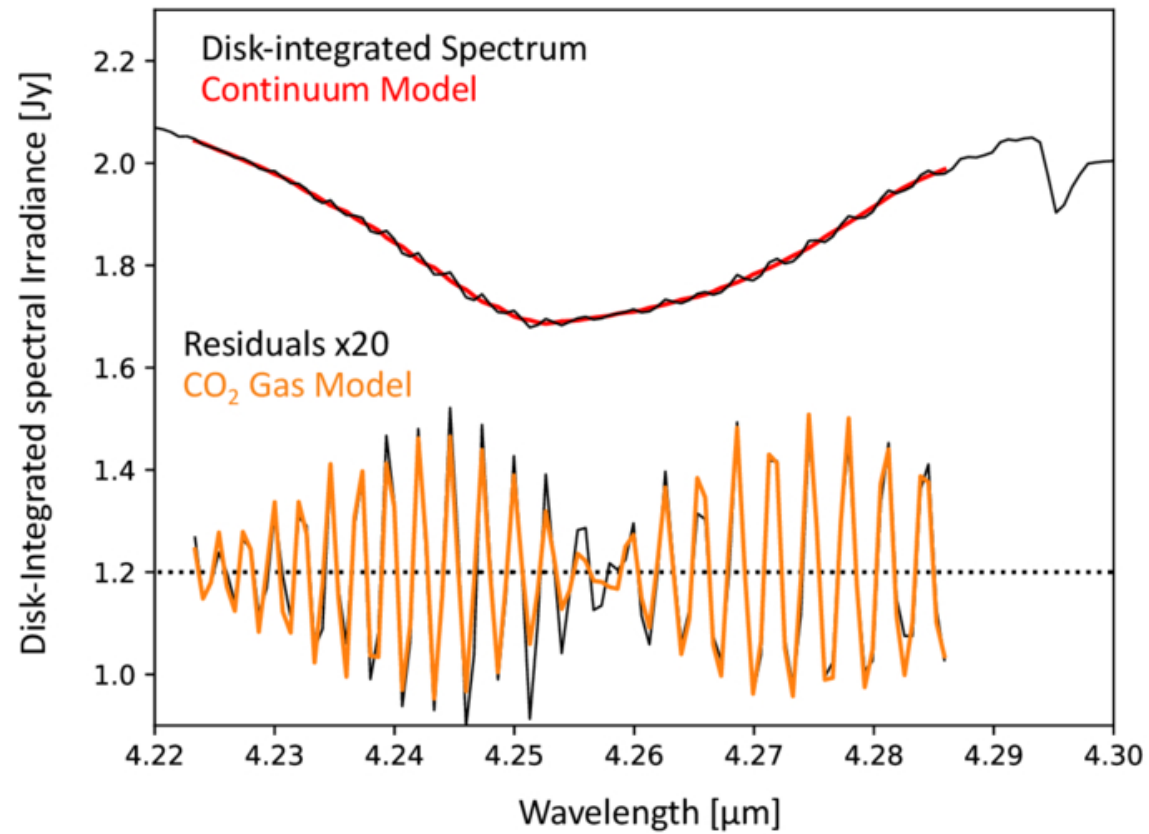
Figure 5. from Maria Camarca et al 2026 Planet. Sci. J. 7 doi:10.3847/PSJ/ae9608 https://dx.doi.org/10.3847/PSJ/ae9608 © 2026. The Author(s). Published by the American Astronomical Society.
