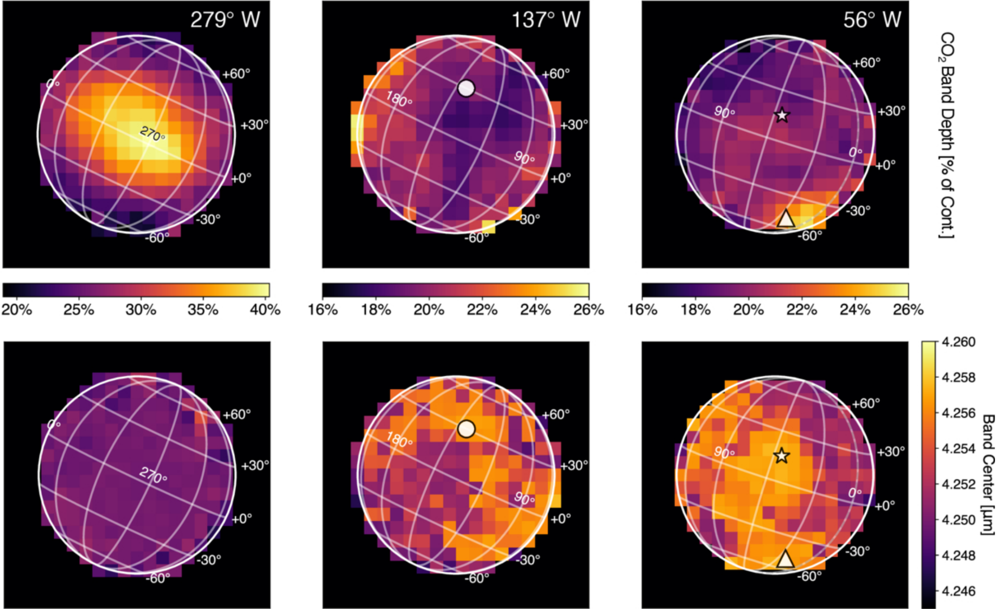
Figure 4. from Maria Camarca et al 2026 Planet. Sci. J. 7 doi:10.3847/PSJ/ae9608 https://dx.doi.org/10.3847/PSJ/ae9608 © 2026. The Author(s). Published by the American Astronomical Society.
