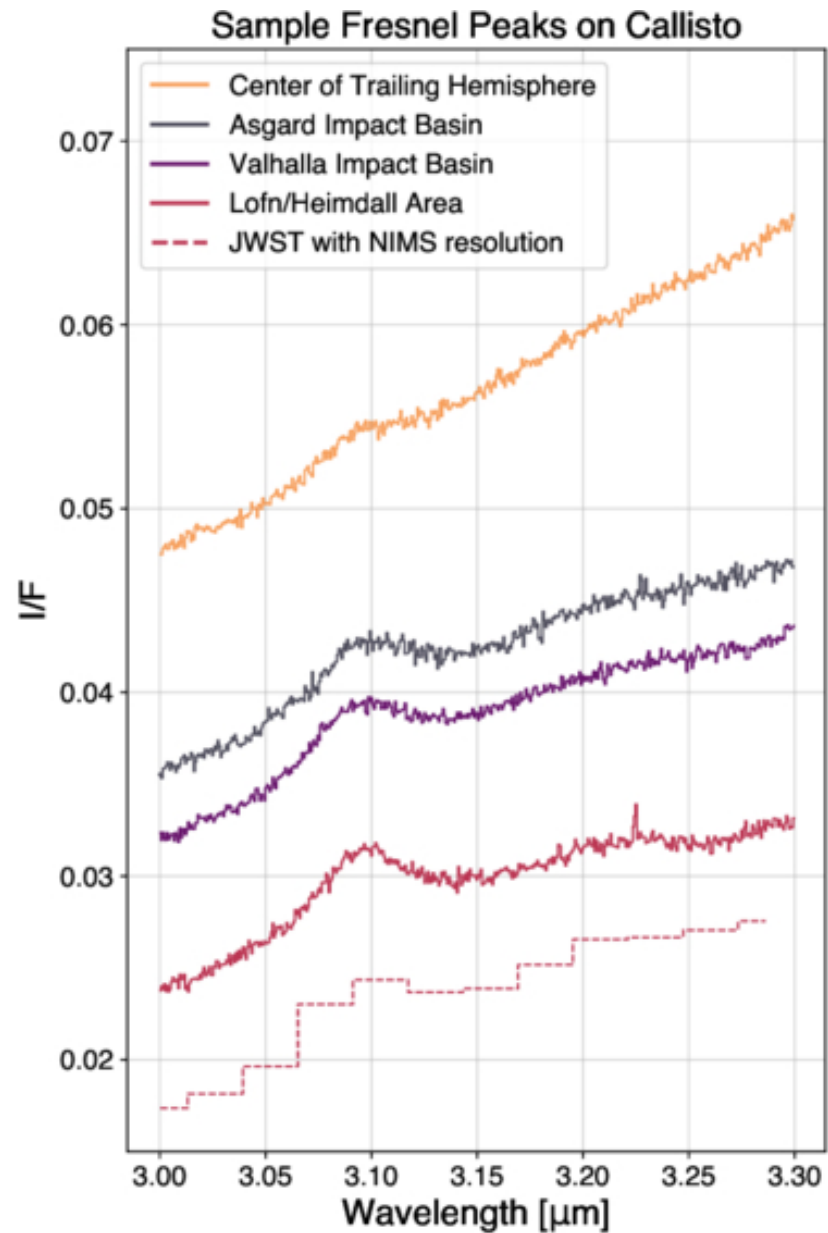
Figure 3. from Maria Camarca et al 2026 Planet. Sci. J. 7 doi:10.3847/PSJ/ae9608 https://dx.doi.org/10.3847/PSJ/ae9608 © 2026. The Author(s). Published by the American Astronomical Society.
