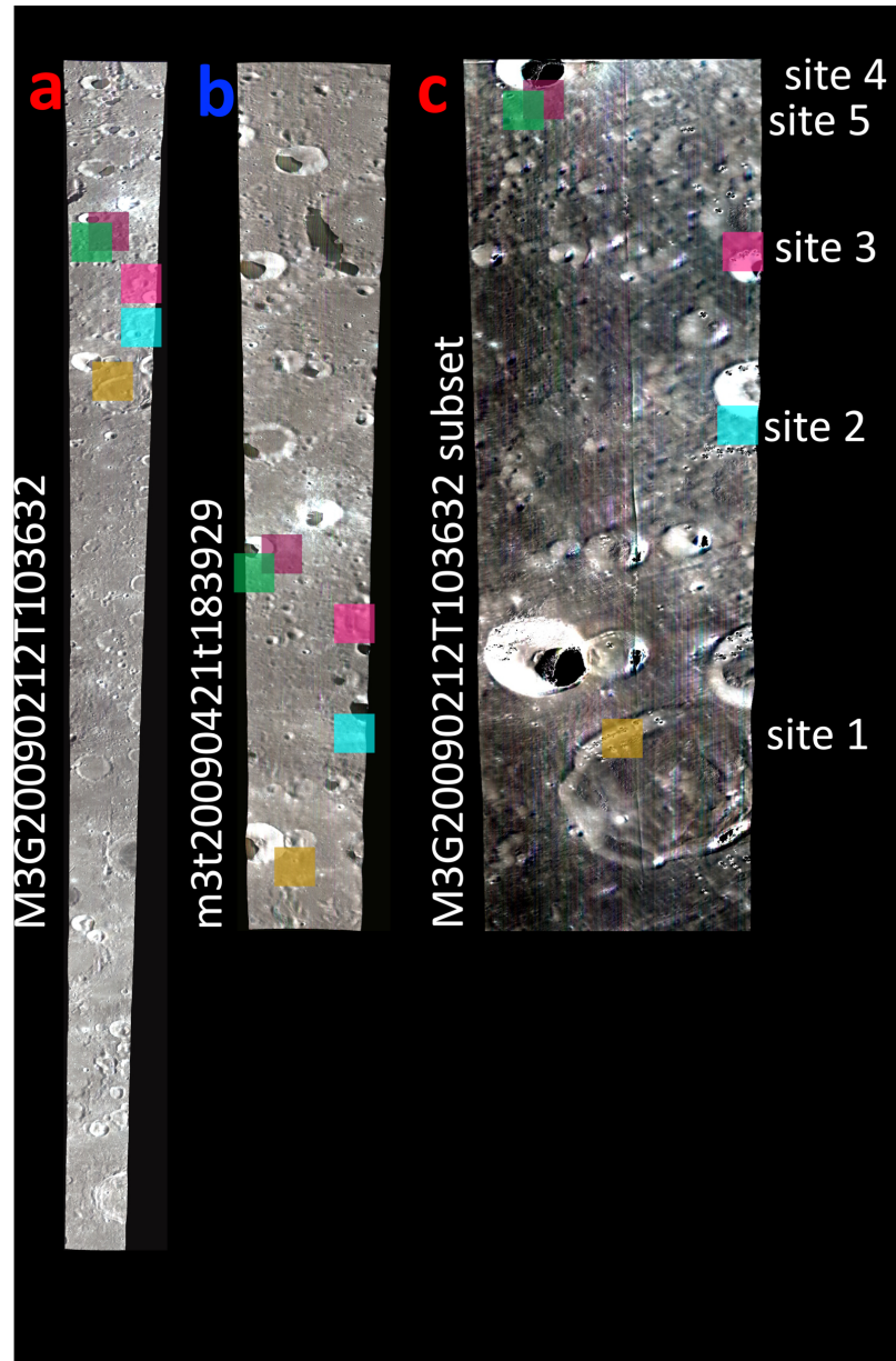
Figure 2. from Angela M. Dapremont et al 2026 Planet. Sci. J. 7 doi:10.3847/PSJ/ae953c https://dx.doi.org/10.3847/PSJ/ae953c © 2026. The Author(s). Published by the American Astronomical Society.
