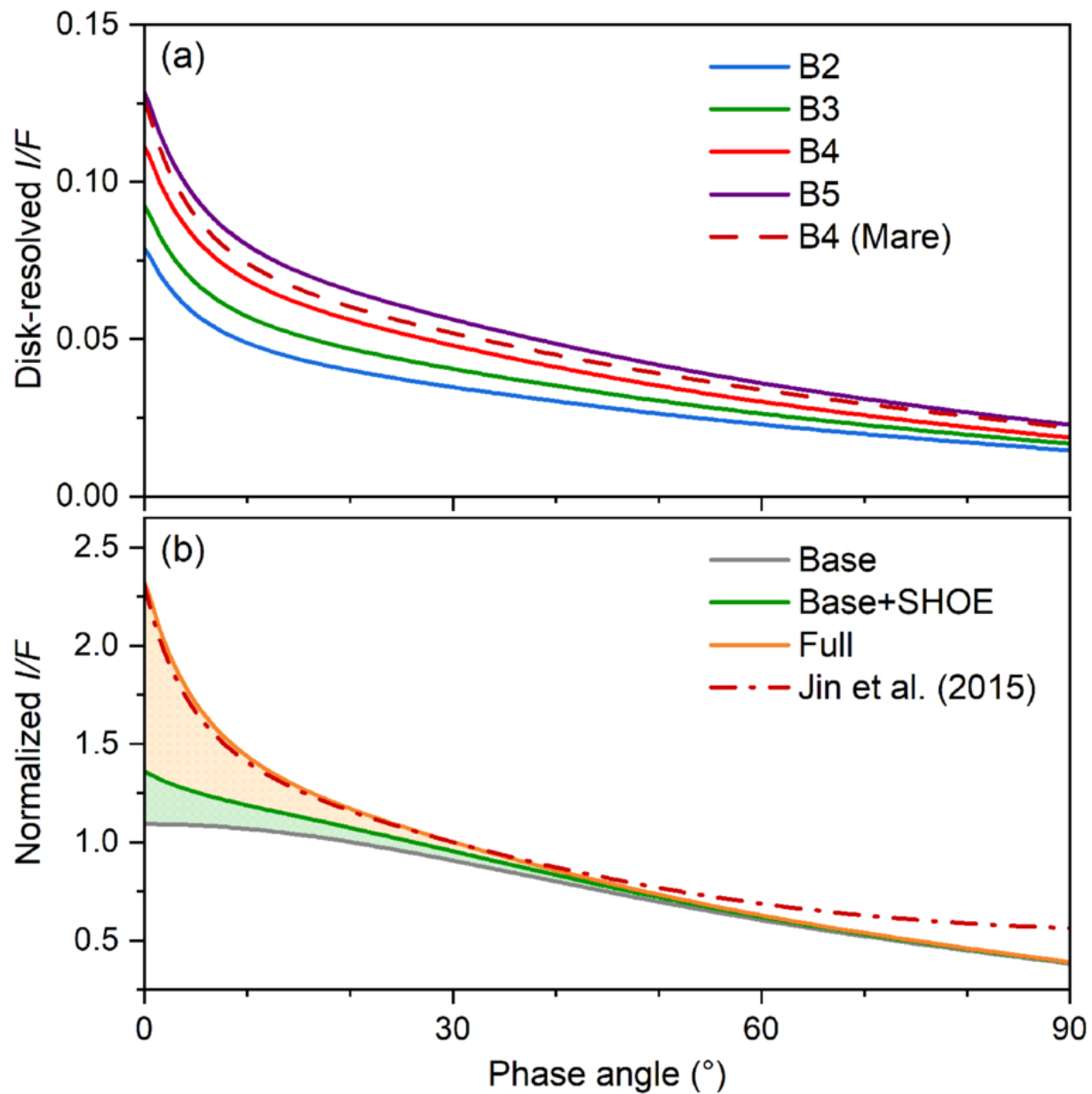
Figure 7. from Siyuan Li et al 2026 Planet. Sci. J. 7 doi:10.3847/PSJ/ae93ab https://dx.doi.org/10.3847/PSJ/ae93ab © 2026. The Author(s). Published by the American Astronomical Society.
