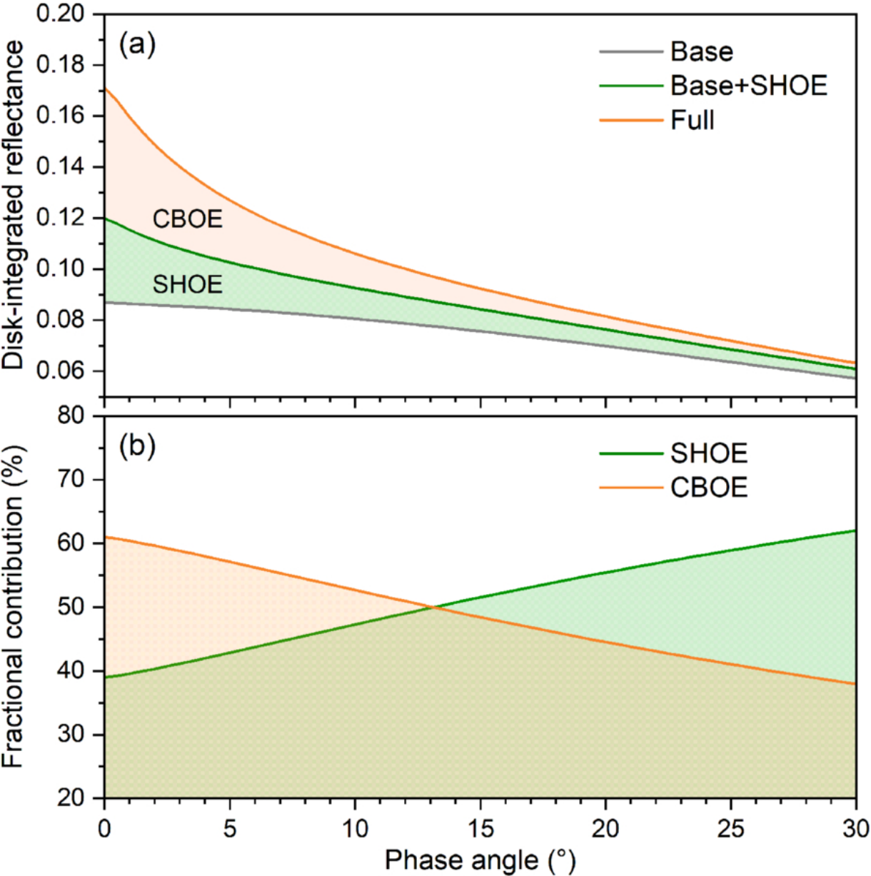
Figure 5. from Siyuan Li et al 2026 Planet. Sci. J. 7 doi:10.3847/PSJ/ae93ab https://dx.doi.org/10.3847/PSJ/ae93ab © 2026. The Author(s). Published by the American Astronomical Society.
