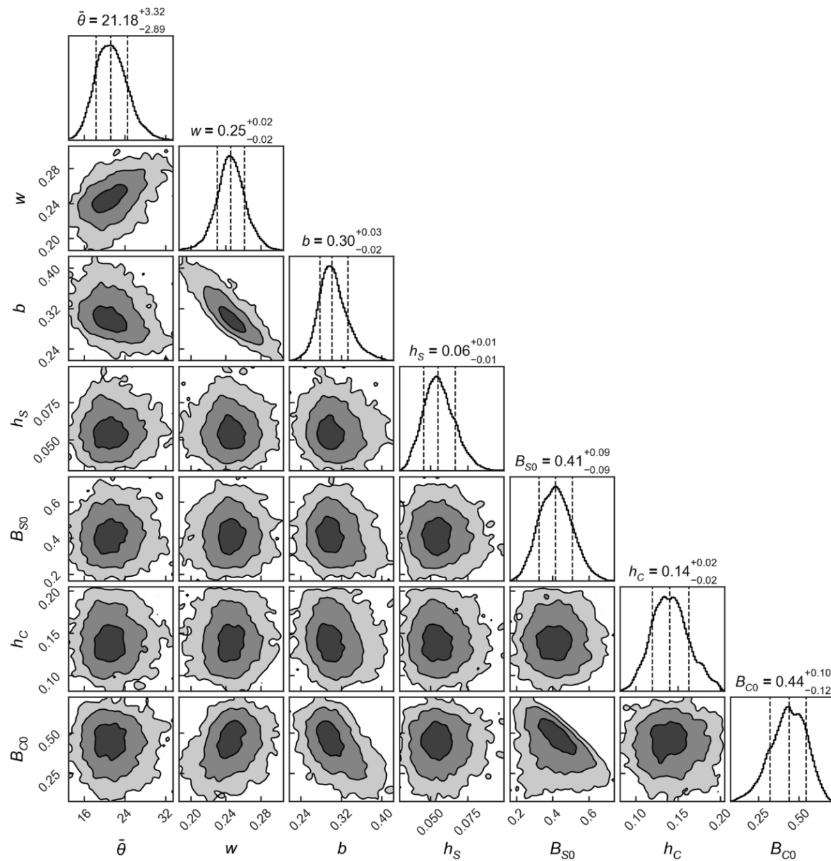
Figure 4. Posterior diagnostic corner plots from Siyuan Li et al 2026 Planet. Sci. J. 7 doi:10.3847/PSJ/ae93ab https://dx.doi.org/10.3847/PSJ/ae93ab © 2026. The Author(s). Published by the American Astronomical Society.
