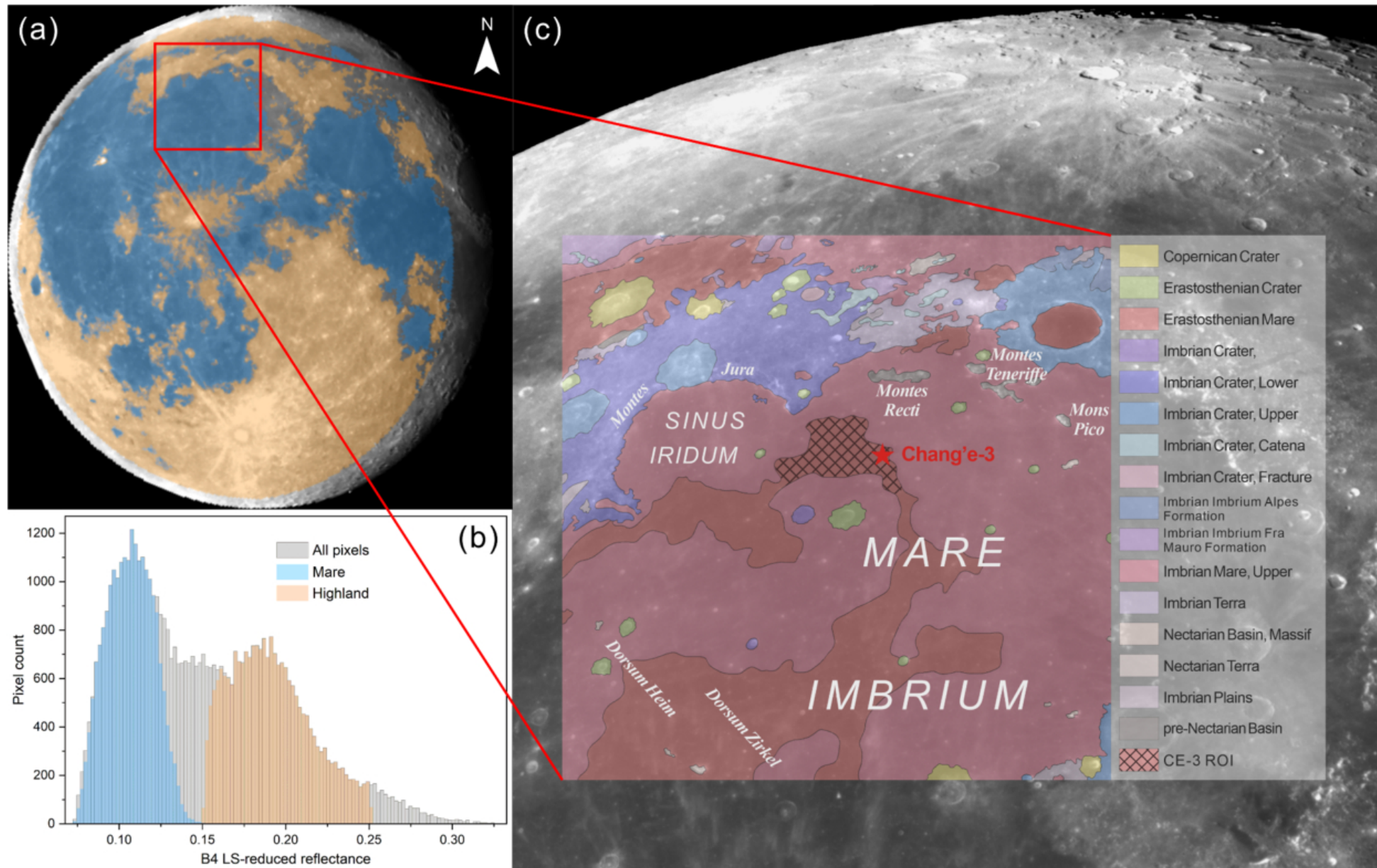
Figure 2. from Siyuan Li et al 2026 Planet. Sci. J. 7 doi:10.3847/PSJ/ae93ab https://dx.doi.org/10.3847/PSJ/ae93ab © 2026. The Author(s). Published by the American Astronomical Society.
