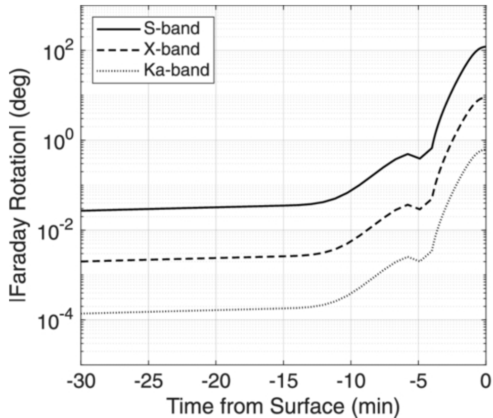
Figure 7. from Seho Kim et al 2026 Planet. Sci. J. 7 doi:10.3847/PSJ/ae939c https://dx.doi.org/10.3847/PSJ/ae939c © 2026. The Author(s). Published by the American Astronomical Society.
