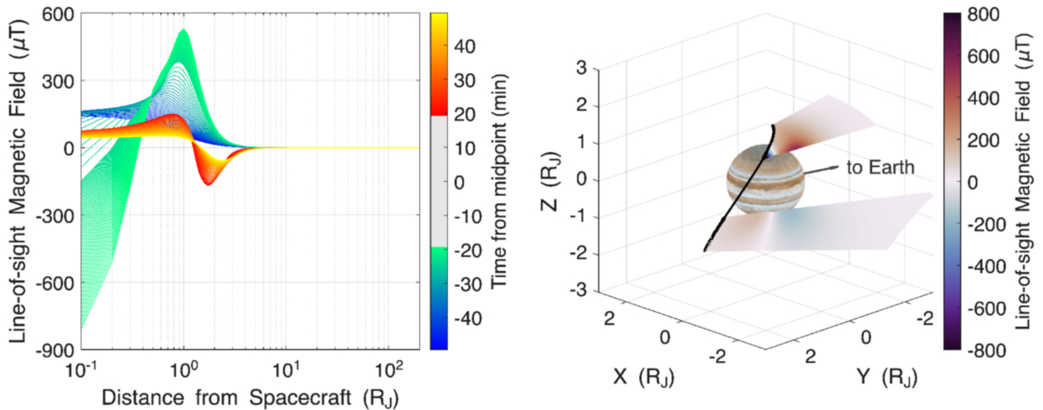
Figure 5. from Seho Kim et al 2026 Planet. Sci. J. 7 doi:10.3847/PSJ/ae939c https://dx.doi.org/10.3847/PSJ/ae939c © 2026. The Author(s). Published by the American Astronomical Society.
