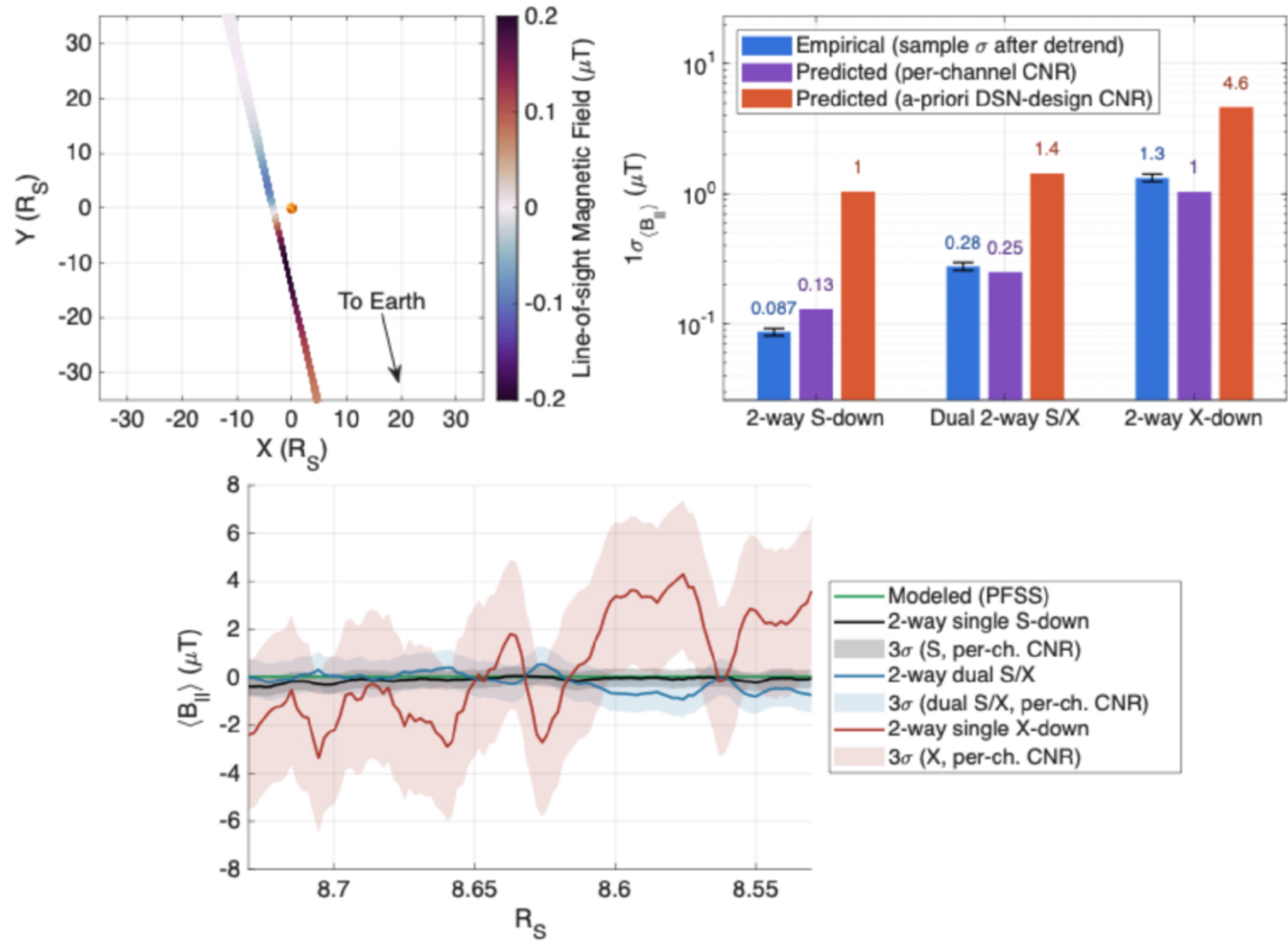
Figure 4. from Seho Kim et al 2026 Planet. Sci. J. 7 doi:10.3847/PSJ/ae939c https://dx.doi.org/10.3847/PSJ/ae939c © 2026. The Author(s). Published by the American Astronomical Society.
