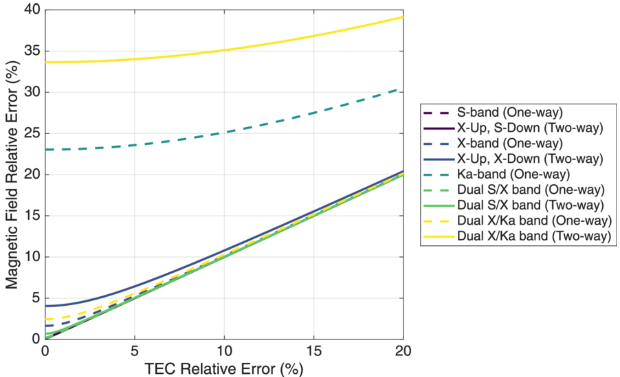
Figure 3. from Seho Kim et al 2026 Planet. Sci. J. 7 doi:10.3847/PSJ/ae939c https://dx.doi.org/10.3847/PSJ/ae939c © 2026. The Author(s). Published by the American Astronomical Society.
