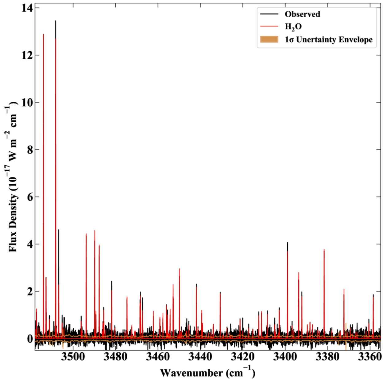
Figure 8. from Nathan X. Roth et al 2026 Planet. Sci. J. 7 doi:10.3847/PSJ/ae91ed https://dx.doi.org/10.3847/PSJ/ae91ed © 2026. The Author(s). Published by the American Astronomical Society.
