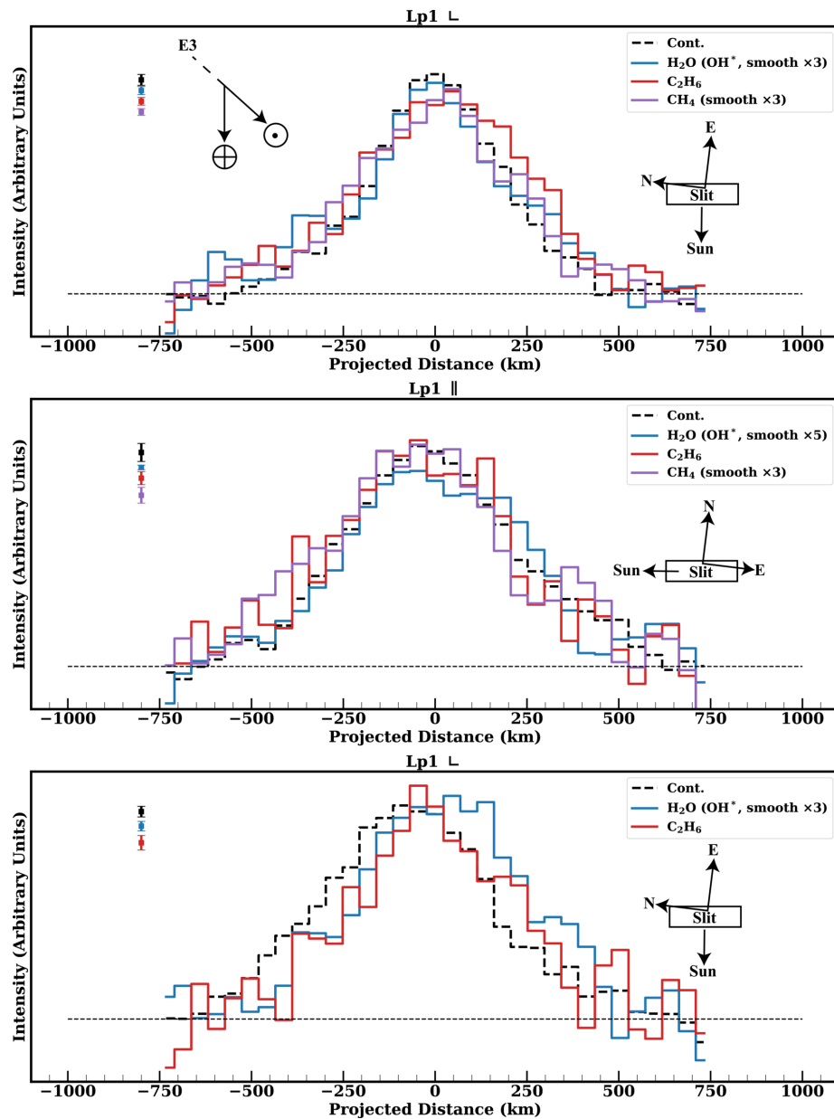
Figure 7. from Nathan X. Roth et al 2026 Planet. Sci. J. 7 doi:10.3847/PSJ/ae91ed https://dx.doi.org/10.3847/PSJ/ae91ed © 2026. The Author(s). Published by the American Astronomical Society.
