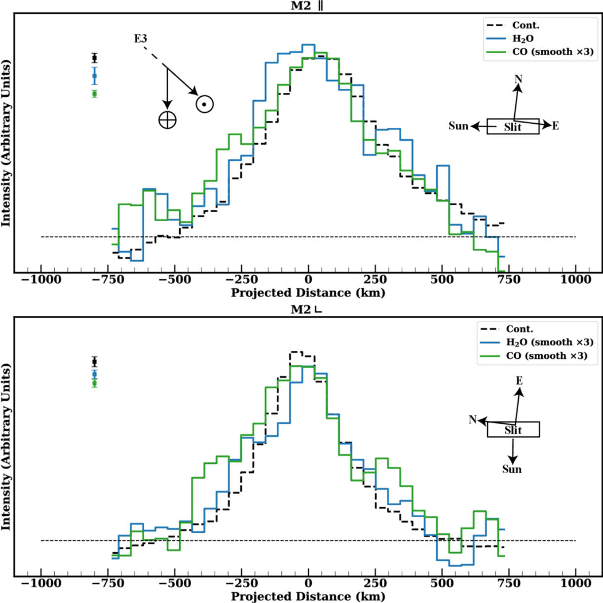
Figure 6. from Nathan X. Roth et al 2026 Planet. Sci. J. 7 doi:10.3847/PSJ/ae91ed https://dx.doi.org/10.3847/PSJ/ae91ed © 2026. The Author(s). Published by the American Astronomical Society.
