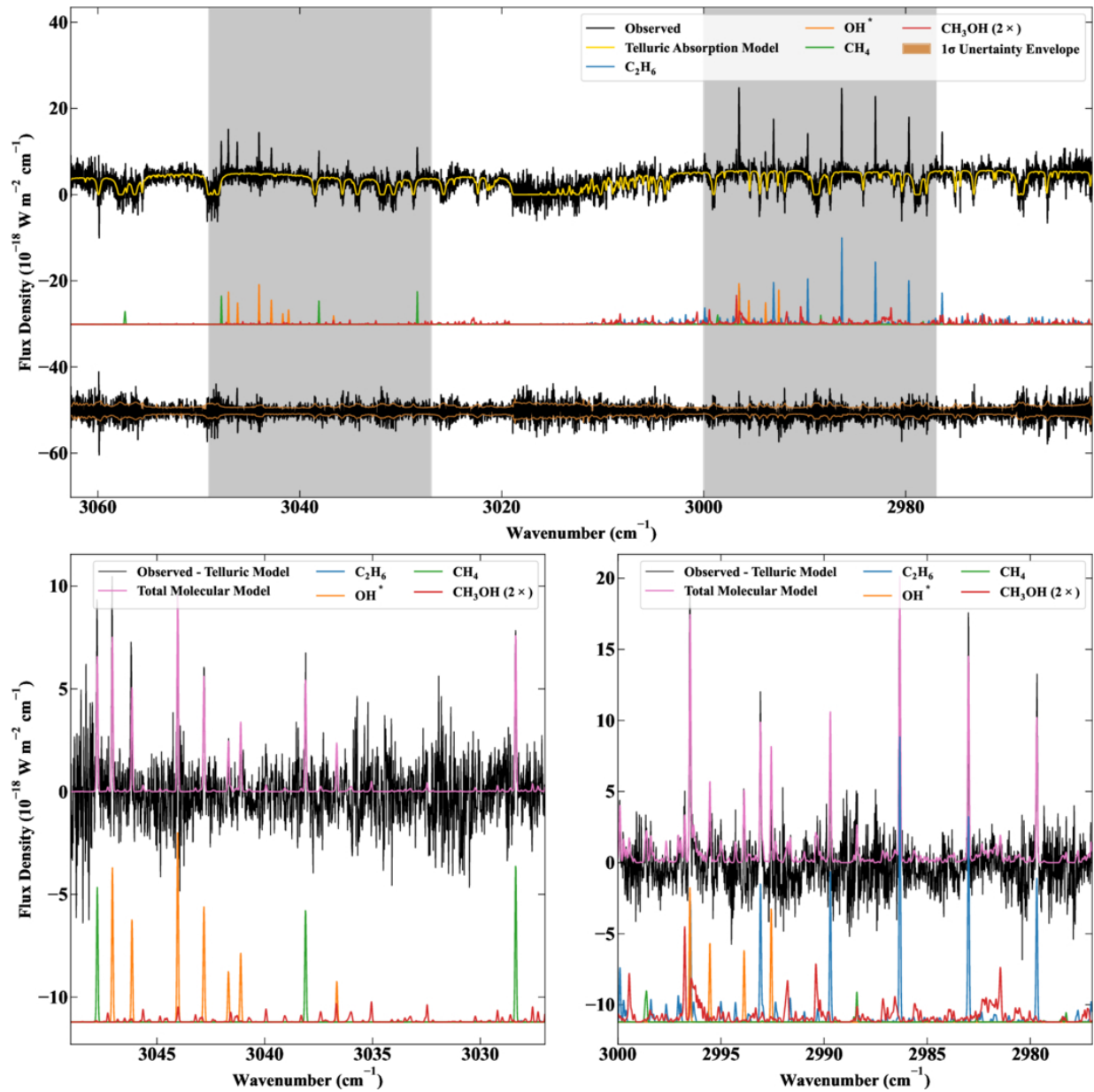
Figure 3. from Nathan X. Roth et al 2026 Planet. Sci. J. 7 doi:10.3847/PSJ/ae91ed https://dx.doi.org/10.3847/PSJ/ae91ed © 2026. The Author(s). Published by the American Astronomical Society.
