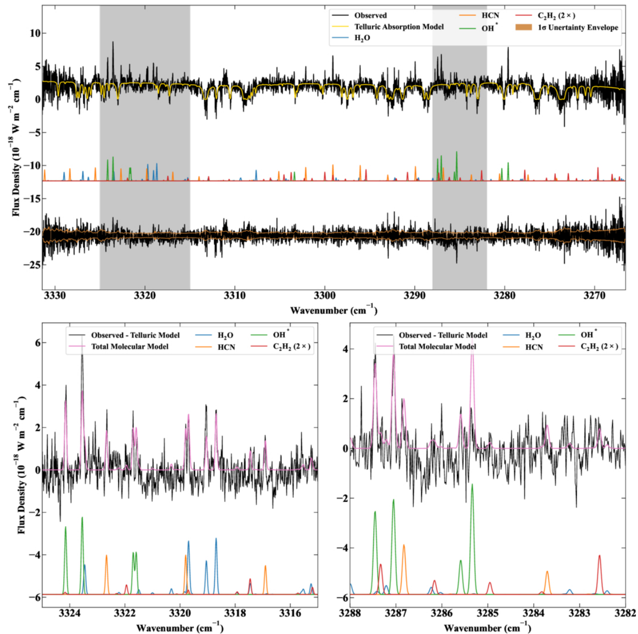
Figure 1. from Nathan X. Roth et al 2026 Planet. Sci. J. 7 doi:10.3847/PSJ/ae91ed https://dx.doi.org/10.3847/PSJ/ae91ed © 2026. The Author(s). Published by the American Astronomical Society.
