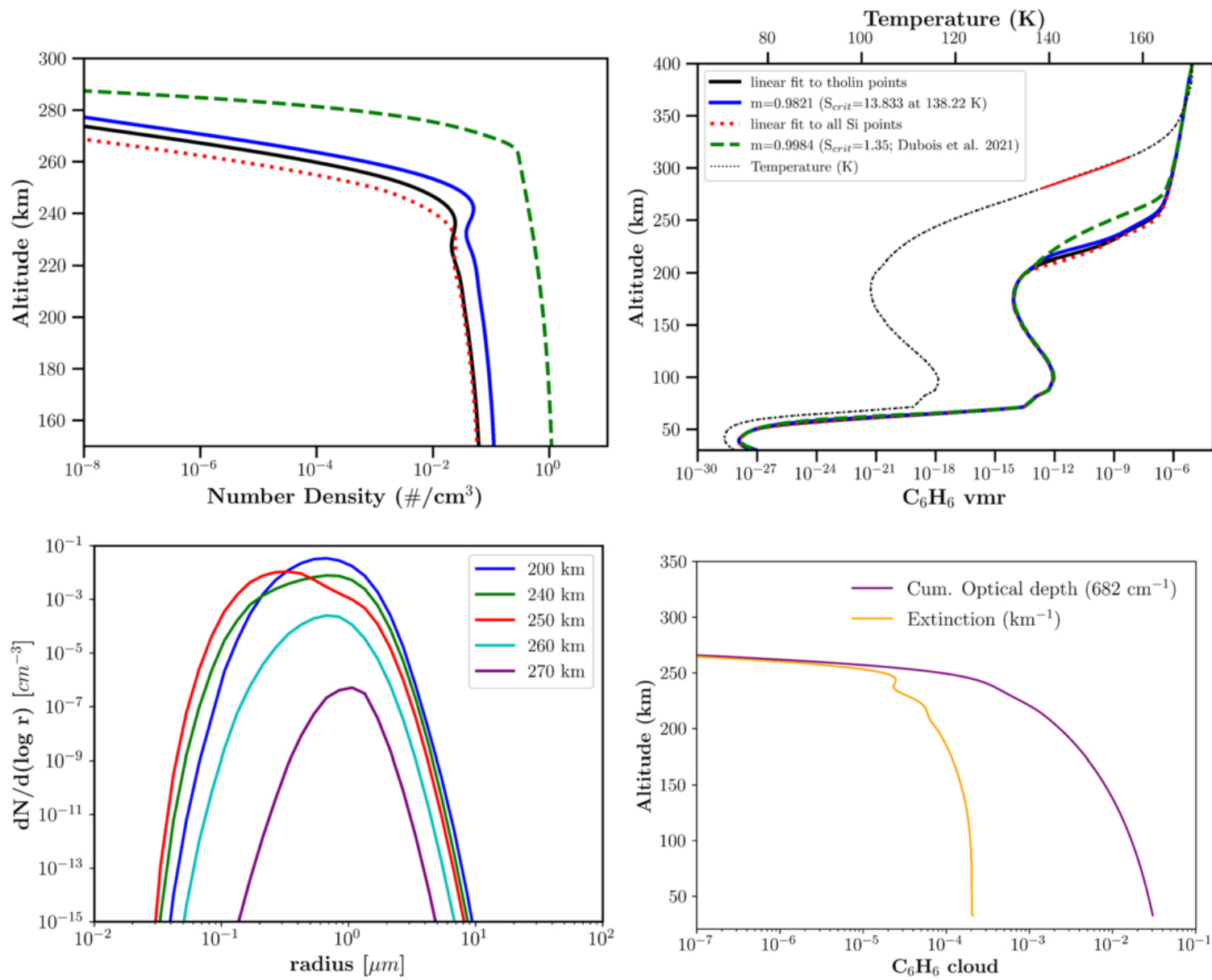
Figure 7. from David Dubois et al 2026 Planet. Sci. J. 7 doi:10.3847/PSJ/ae9092 https://dx.doi.org/10.3847/PSJ/ae9092 © 2026. The Author(s). Published by the American Astronomical Society.
