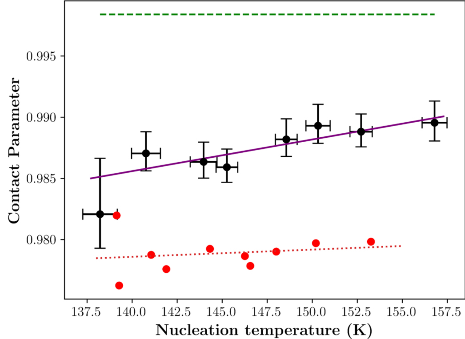
Figure 6. from David Dubois et al 2026 Planet. Sci. J. 7 doi:10.3847/PSJ/ae9092 https://dx.doi.org/10.3847/PSJ/ae9092 © 2026. The Author(s). Published by the American Astronomical Society.
