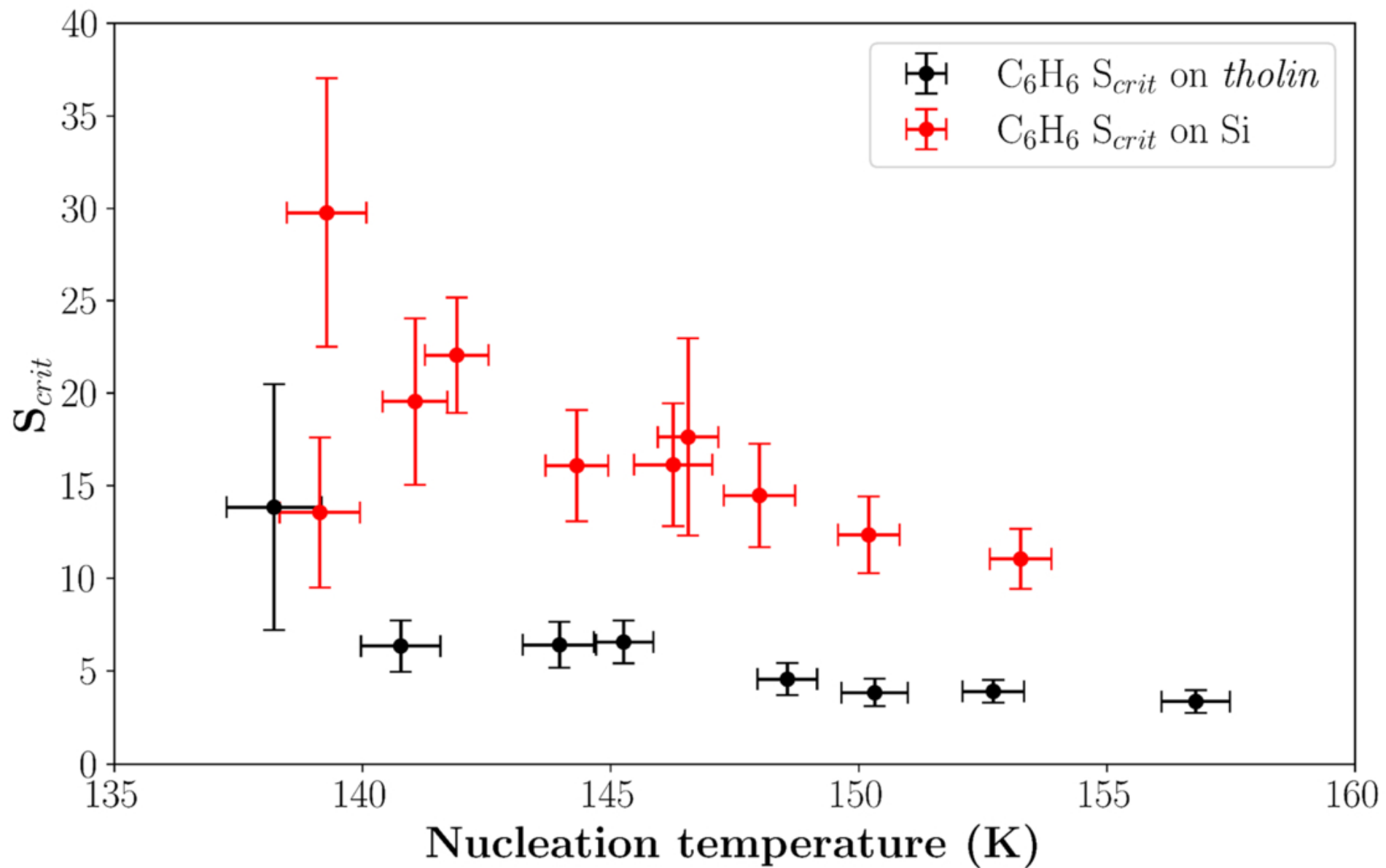
Figure 5. from David Dubois et al 2026 Planet. Sci. J. 7 doi:10.3847/PSJ/ae9092 https://dx.doi.org/10.3847/PSJ/ae9092 © 2026. The Author(s). Published by the American Astronomical Society.
