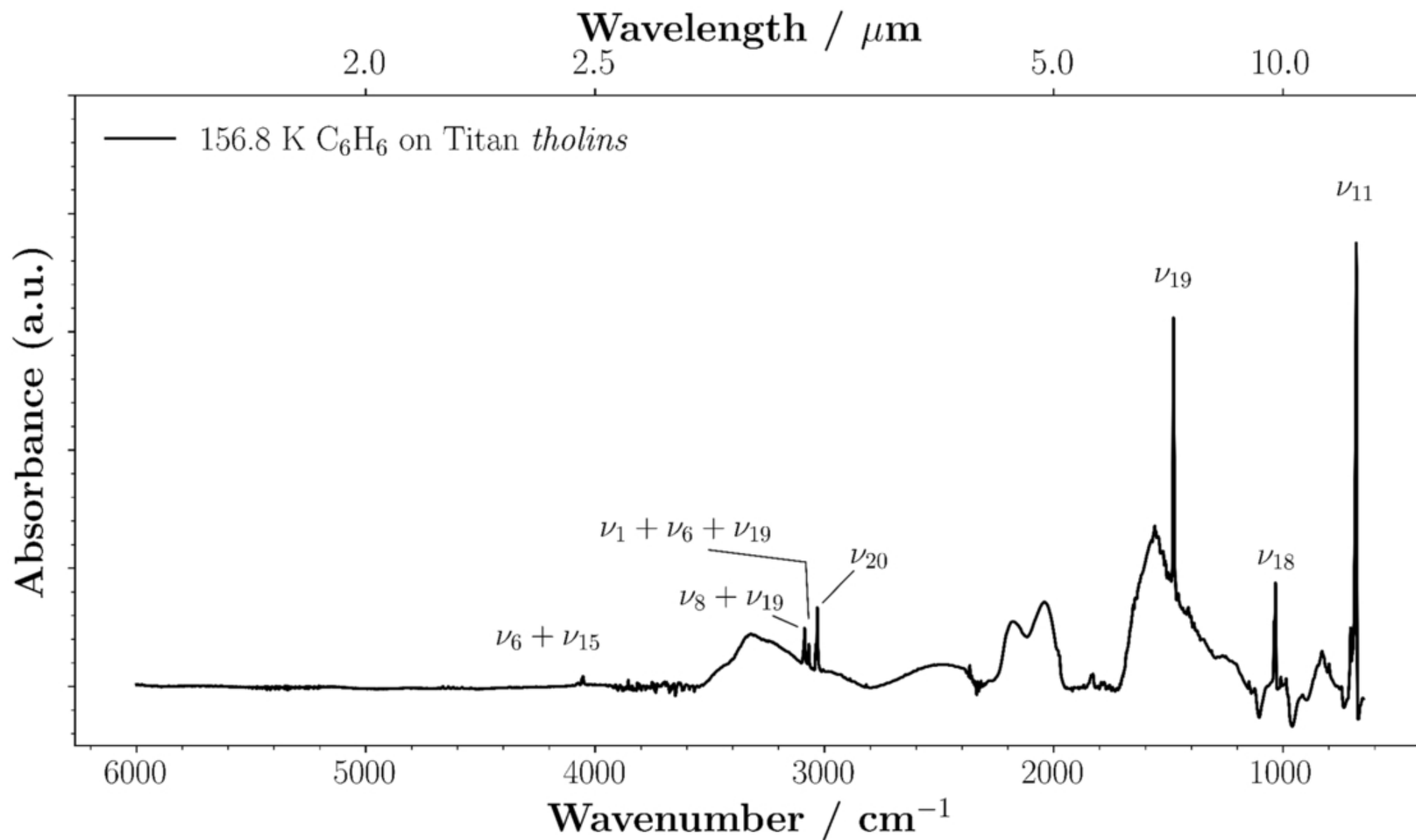
Figure 3. from David Dubois et al 2026 Planet. Sci. J. 7 doi:10.3847/PSJ/ae9092 https://dx.doi.org/10.3847/PSJ/ae9092 © 2026. The Author(s). Published by the American Astronomical Society.
