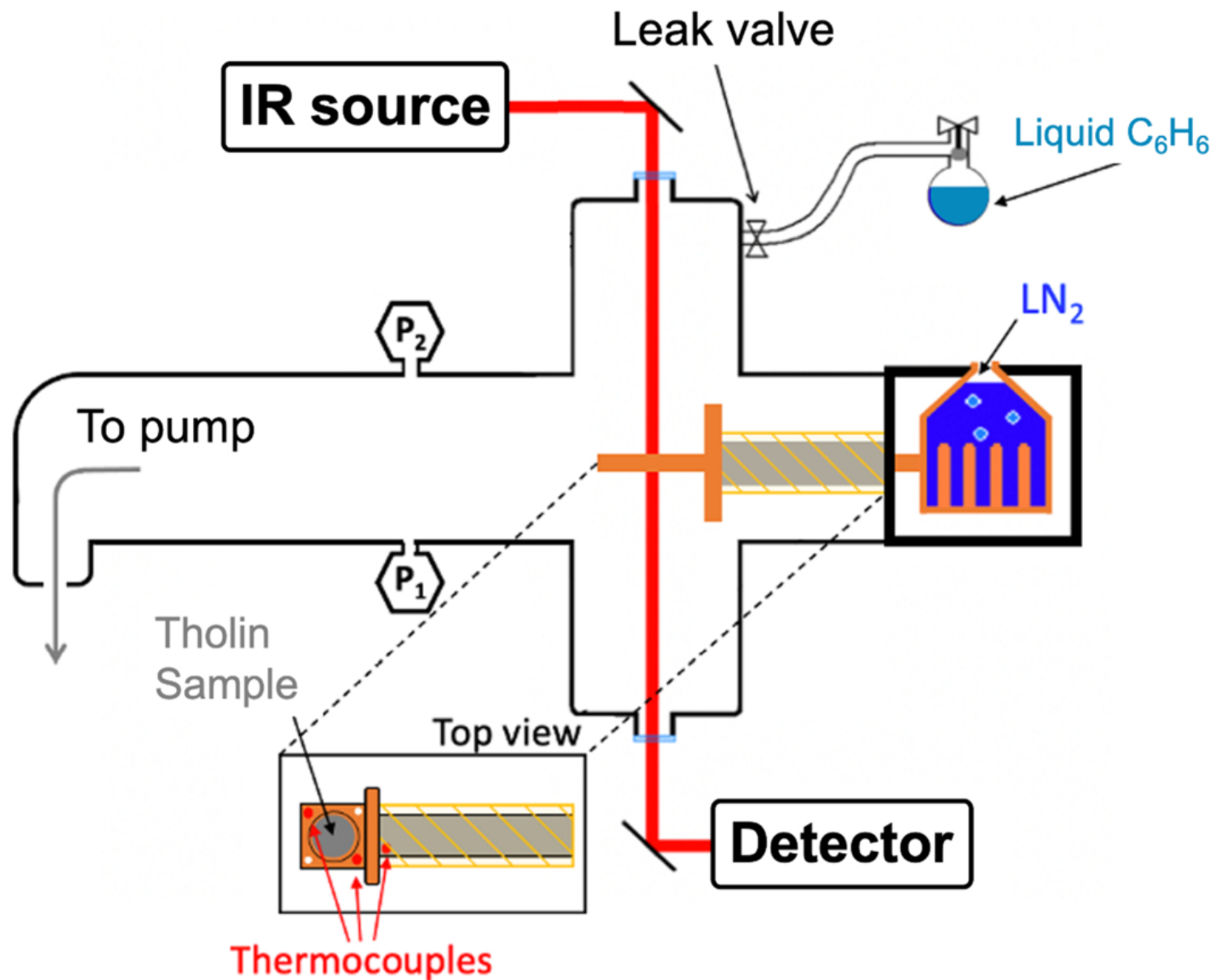
Figure 2. from David Dubois et al 2026 Planet. Sci. J. 7 doi:10.3847/PSJ/ae9092 https://dx.doi.org/10.3847/PSJ/ae9092 © 2026. The Author(s). Published by the American Astronomical Society.
