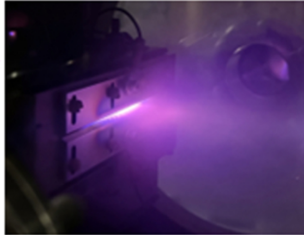
Figure 1. from David Dubois et al 2026 Planet. Sci. J. 7 doi:10.3847/PSJ/ae9092 https://dx.doi.org/10.3847/PSJ/ae9092 © 2026. The Author(s). Published by the American Astronomical Society.
