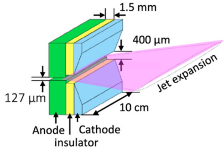
Figure 1. from David Dubois et al 2026 Planet. Sci. J. 7 doi:10.3847/PSJ/ae9092 https://dx.doi.org/10.3847/PSJ/ae9092 © 2026. The Author(s). Published by the American Astronomical Society.
