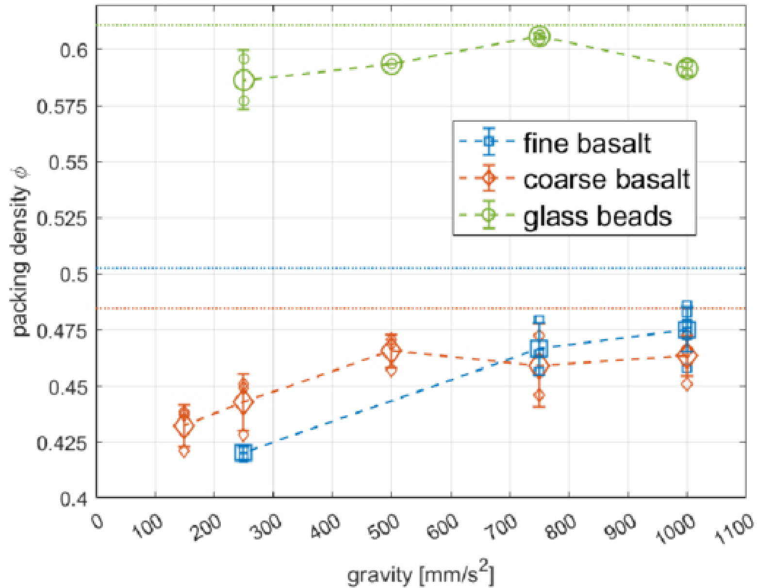
Figure 9. from Matthias Keulen et al 2026 Planet. Sci. J. 7 doi:10.3847/PSJ/ae8fd7 https://dx.doi.org/10.3847/PSJ/ae8fd7 © 2026. The Author(s). Published by the American Astronomical Society.
