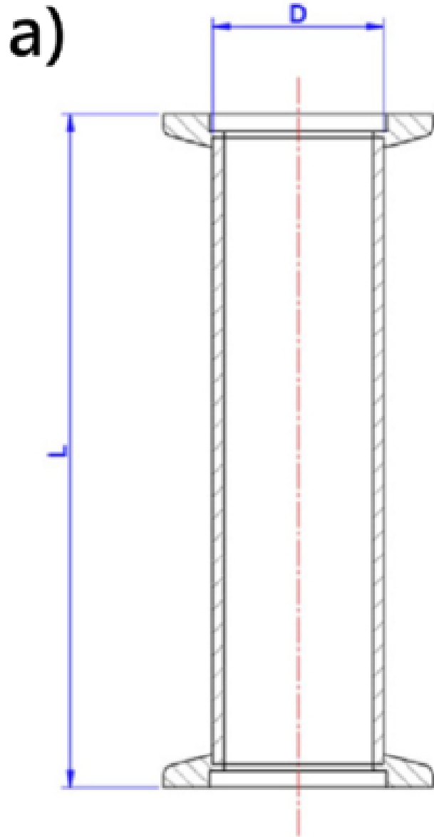
Figure 5. from Matthias Keulen et al 2026 Planet. Sci. J. 7 doi:10.3847/PSJ/ae8fd7 https://dx.doi.org/10.3847/PSJ/ae8fd7 © 2026. The Author(s). Published by the American Astronomical Society.
