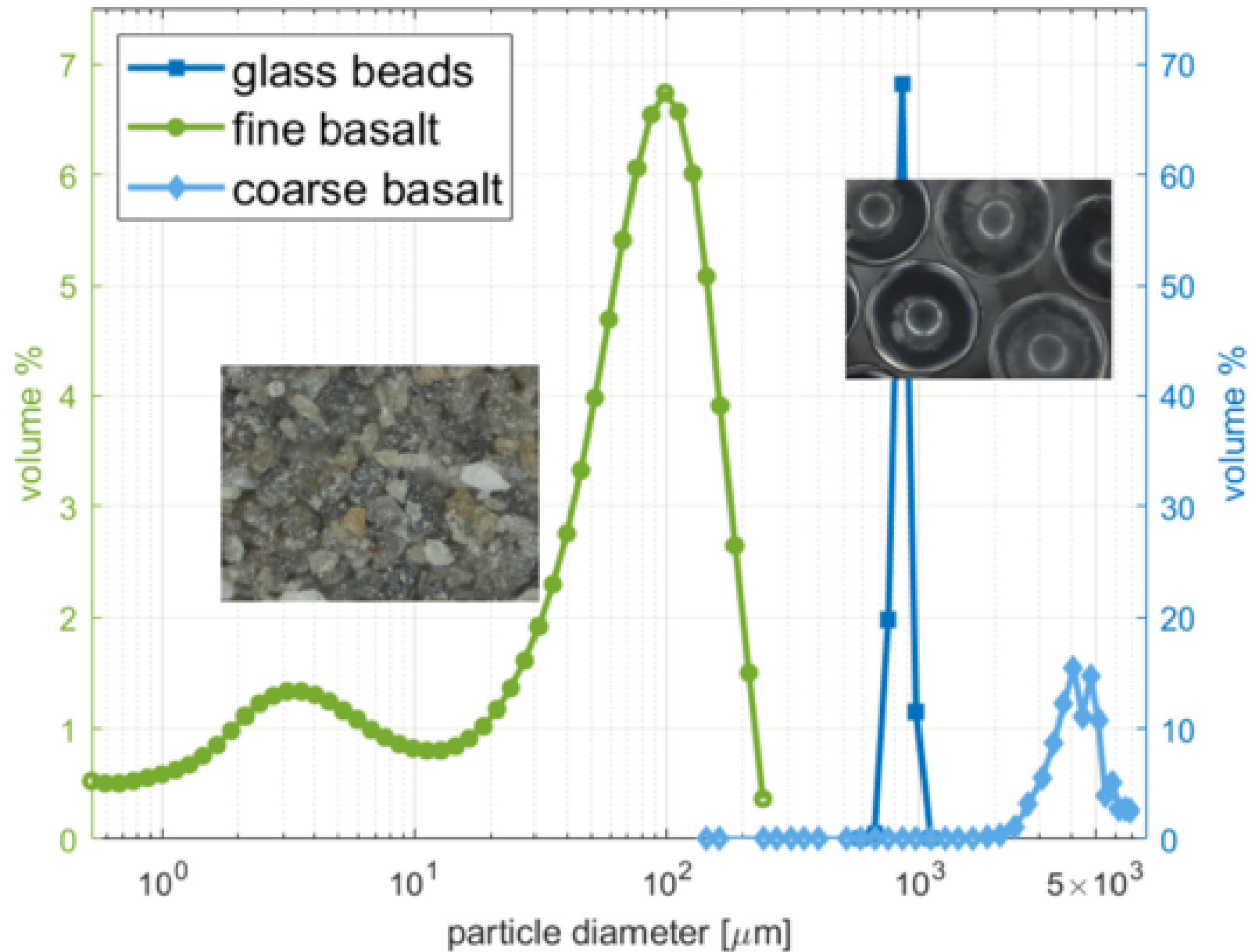
Figure 4. from Matthias Keulen et al 2026 Planet. Sci. J. 7 doi:10.3847/PSJ/ae8fd7 https://dx.doi.org/10.3847/PSJ/ae8fd7 © 2026. The Author(s). Published by the American Astronomical Society.
