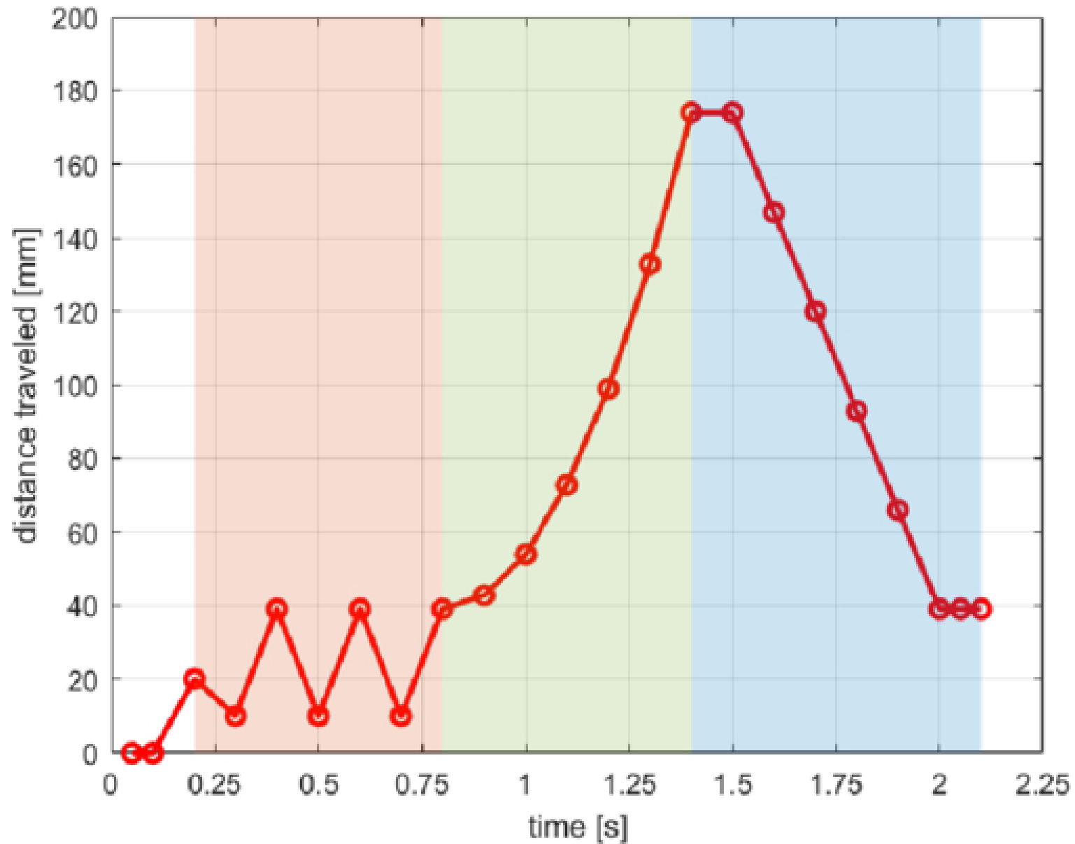
Figure 2. from Matthias Keulen et al 2026 Planet. Sci. J. 7 doi:10.3847/PSJ/ae8fd7 https://dx.doi.org/10.3847/PSJ/ae8fd7 © 2026. The Author(s). Published by the American Astronomical Society.
