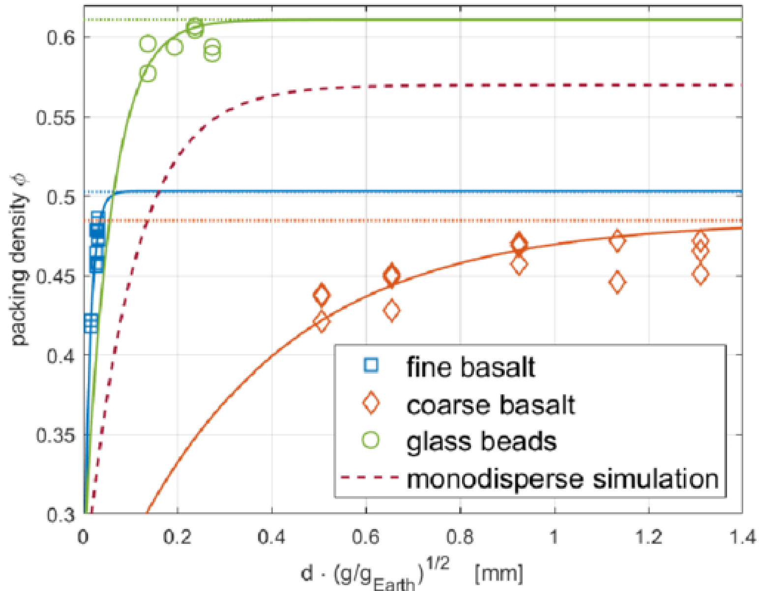
Figure 10. from Matthias Keulen et al 2026 Planet. Sci. J. 7 doi:10.3847/PSJ/ae8fd7 https://dx.doi.org/10.3847/PSJ/ae8fd7 © 2026. The Author(s). Published by the American Astronomical Society.
