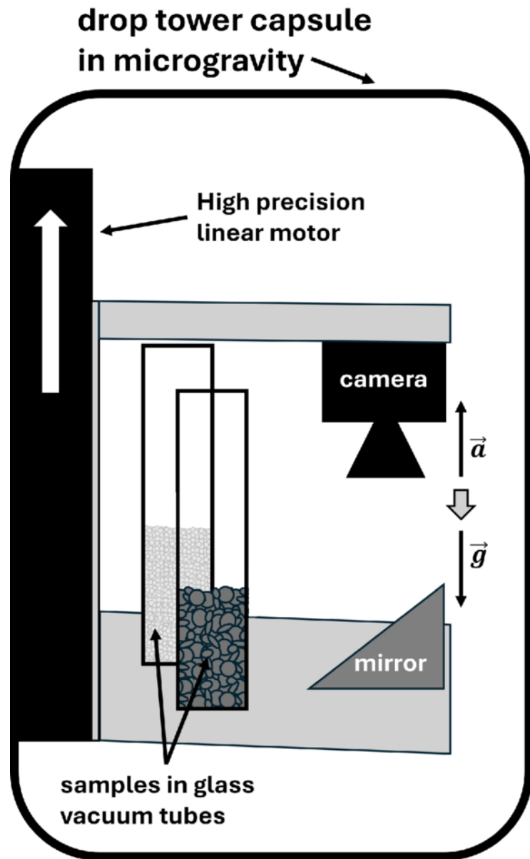
Figure 1. from Matthias Keulen et al 2026 Planet. Sci. J. 7 doi:10.3847/PSJ/ae8fd7 https://dx.doi.org/10.3847/PSJ/ae8fd7 © 2026. The Author(s). Published by the American Astronomical Society.
