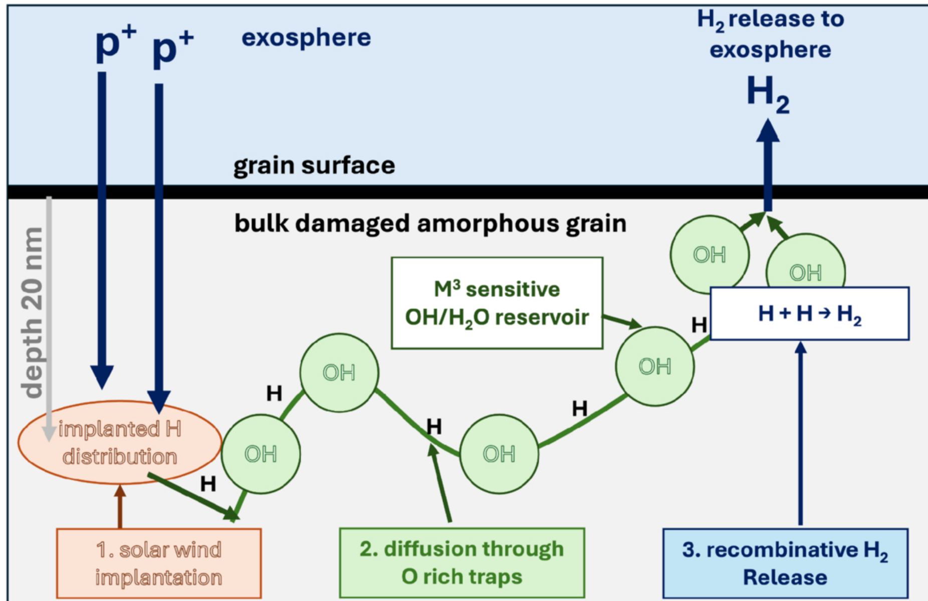
Figure 1. from O. J. Tucker et al 2026 Planet. Sci. J. 7 doi:10.3847/PSJ/ae8e7b https://dx.doi.org/10.3847/PSJ/ae8e7b © 2026. The Author(s). Published by the American Astronomical Society.
