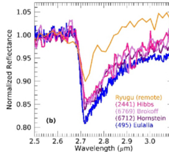
Figure 9. from Lucas T. McClure et al 2026 Planet. Sci. J. 7 doi:10.3847/PSJ/ae8e7a https://dx.doi.org/10.3847/PSJ/ae8e7a © 2026. The Author(s). Published by the American Astronomical Society.
