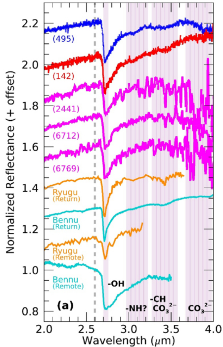
Figure 9. from Lucas T. McClure et al 2026 Planet. Sci. J. 7 doi:10.3847/PSJ/ae8e7a https://dx.doi.org/10.3847/PSJ/ae8e7a © 2026. The Author(s). Published by the American Astronomical Society.
